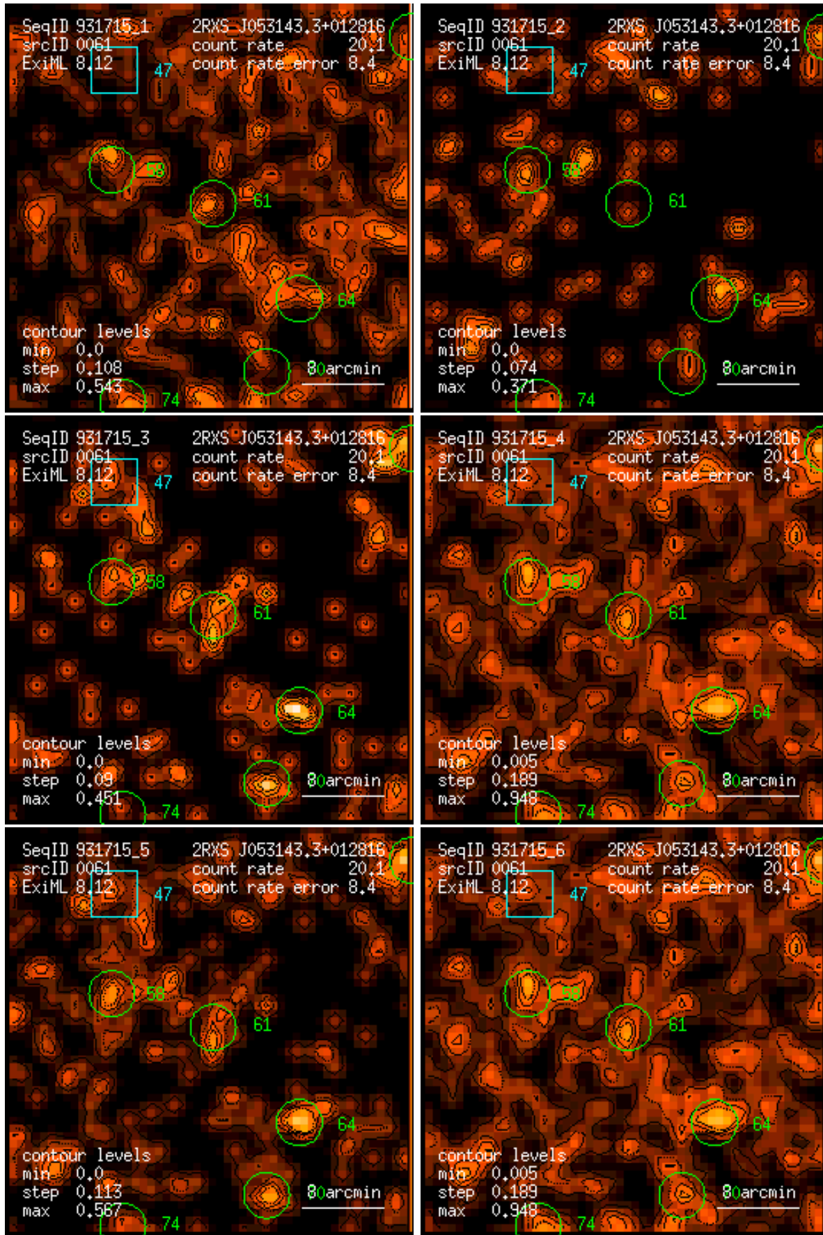
Figure 61: RASS 931715: detection 0061: band rate images, Gaussian filter: (1) PSPC channels 11 – 41, (2) 52 – 90, (3) 91 – 201, (4) 11 – 235, (5) 52 – 201, (6) 11 – 201. Broad band rates in counts/ks. Band rate contour levels in counts/ks/arcmin 2 .
