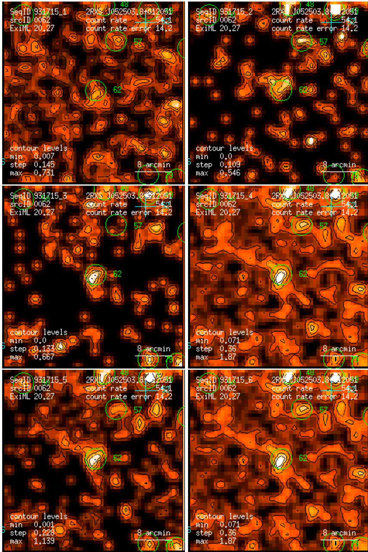
Figure 62: RASS 931715: detection 0062: band rate images, Gaussian filter: (1) PSPC channels 11 – 41, (2) 52 – 90, (3) 91 – 201, (4) 11 – 235, (5) 52 – 201, (6) 11 – 201. Broad band rates in counts/ks. Band rate contour levels in counts/ks/arcmin 2 .
