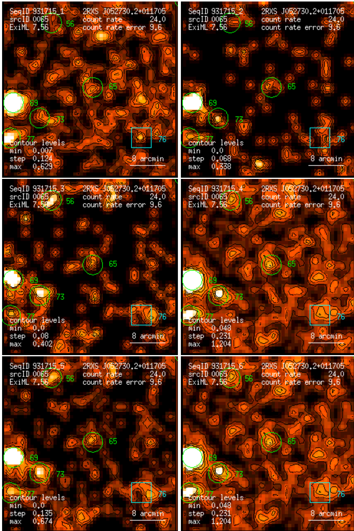
Figure 65: RASS 931715: detection 0065: band rate images, Gaussian filter: (1) PSPC channels 11 – 41, (2) 52 – 90, (3) 91 – 201, (4) 11 – 235, (5) 52 – 201, (6) 11 – 201. Broad band rates in counts/ks. Band rate contour levels in counts/ks/arcmin 2 .
