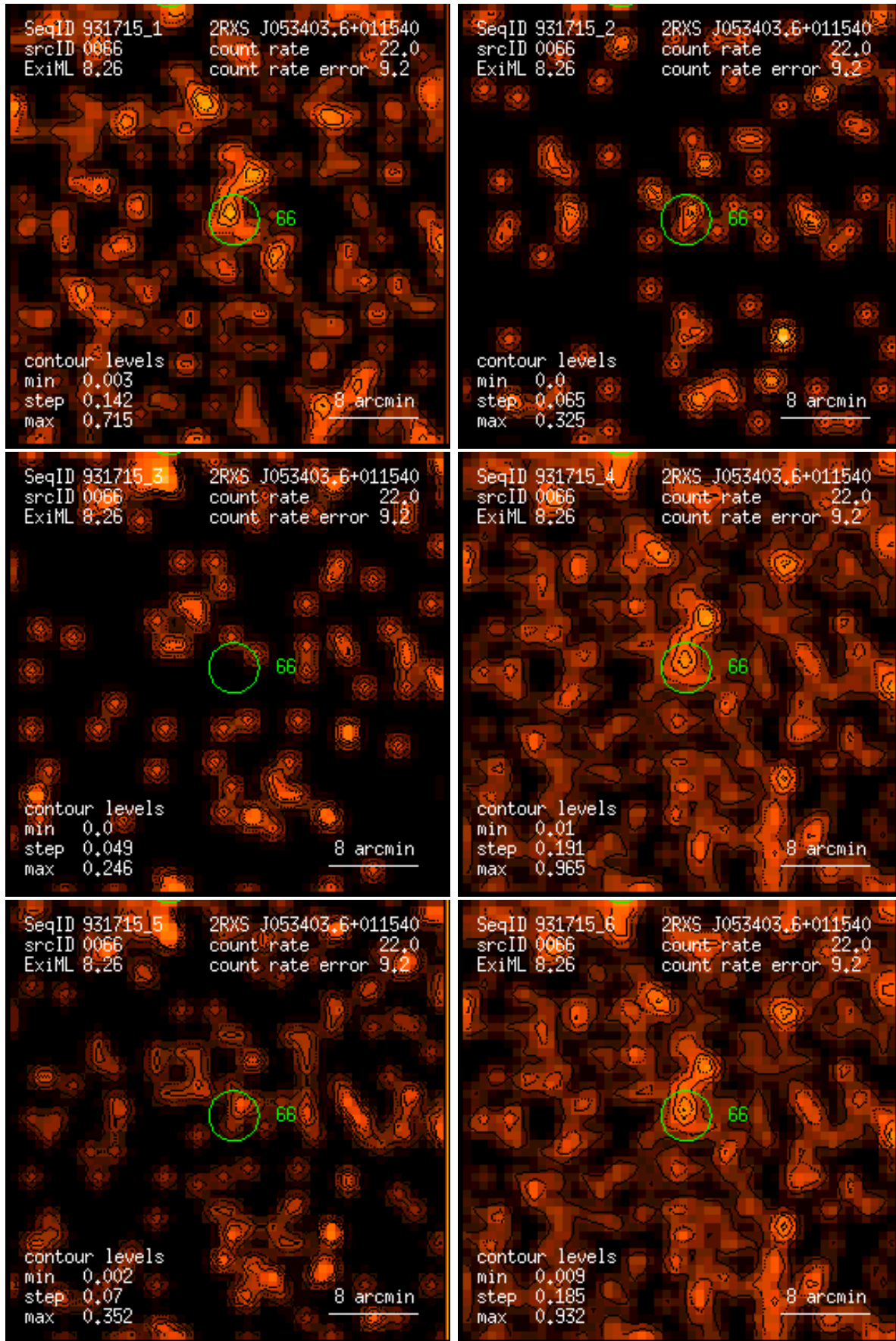
Figure 66: RASS 931715: detection 0066: band rate images, Gaussian filter: (1) PSPC channels 11 – 41, (2) 52 – 90, (3) 91 – 201, (4) 11 – 235, (5) 52 – 201, (6) 11 – 201. Broad band rates in counts/ks. Band rate contour levels in counts/ks/arcmin 2 .
