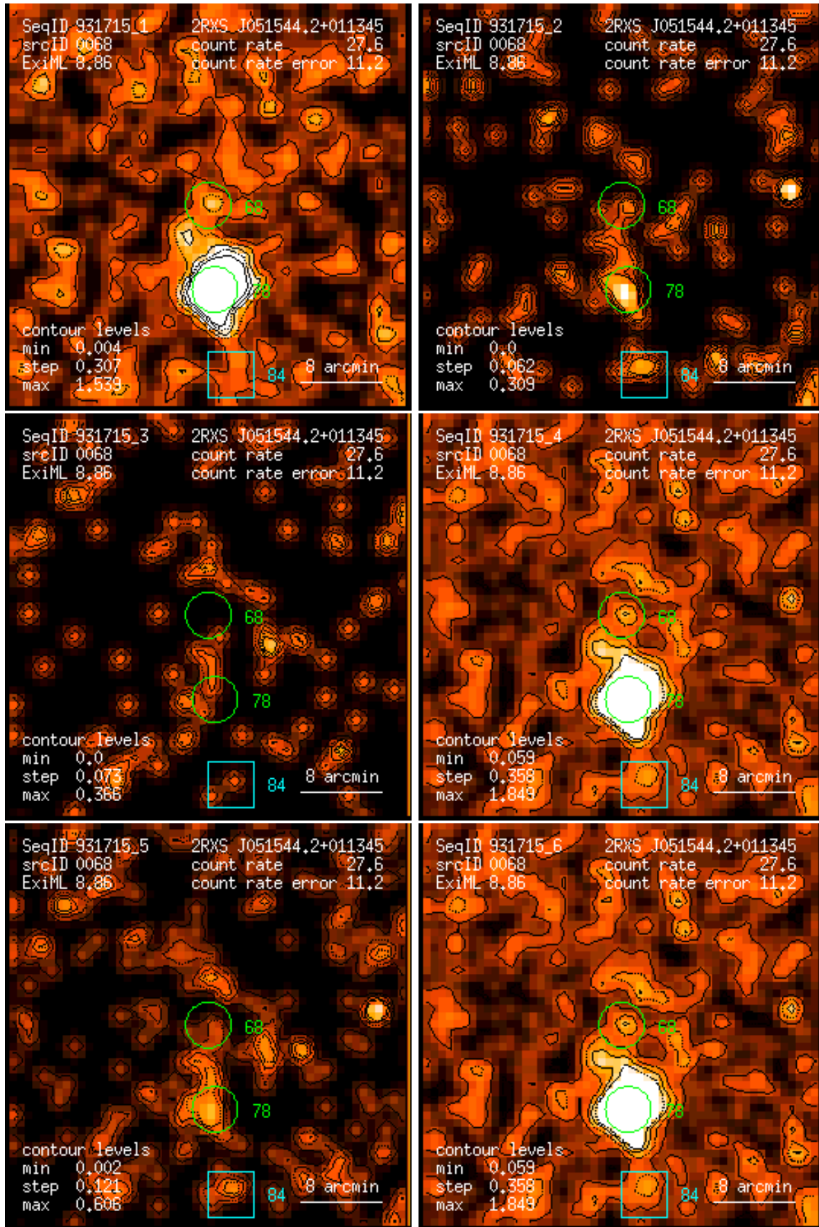
Figure 68: RASS 931715: detection 0068: band rate images, Gaussian filter: (1) PSPC channels 11 – 41, (2) 52 – 90, (3) 91 – 201, (4) 11 – 235, (5) 52 – 201, (6) 11 – 201. Broad band rates in counts/ks. Band rate contour levels in counts/ks/arcmin 2 .
