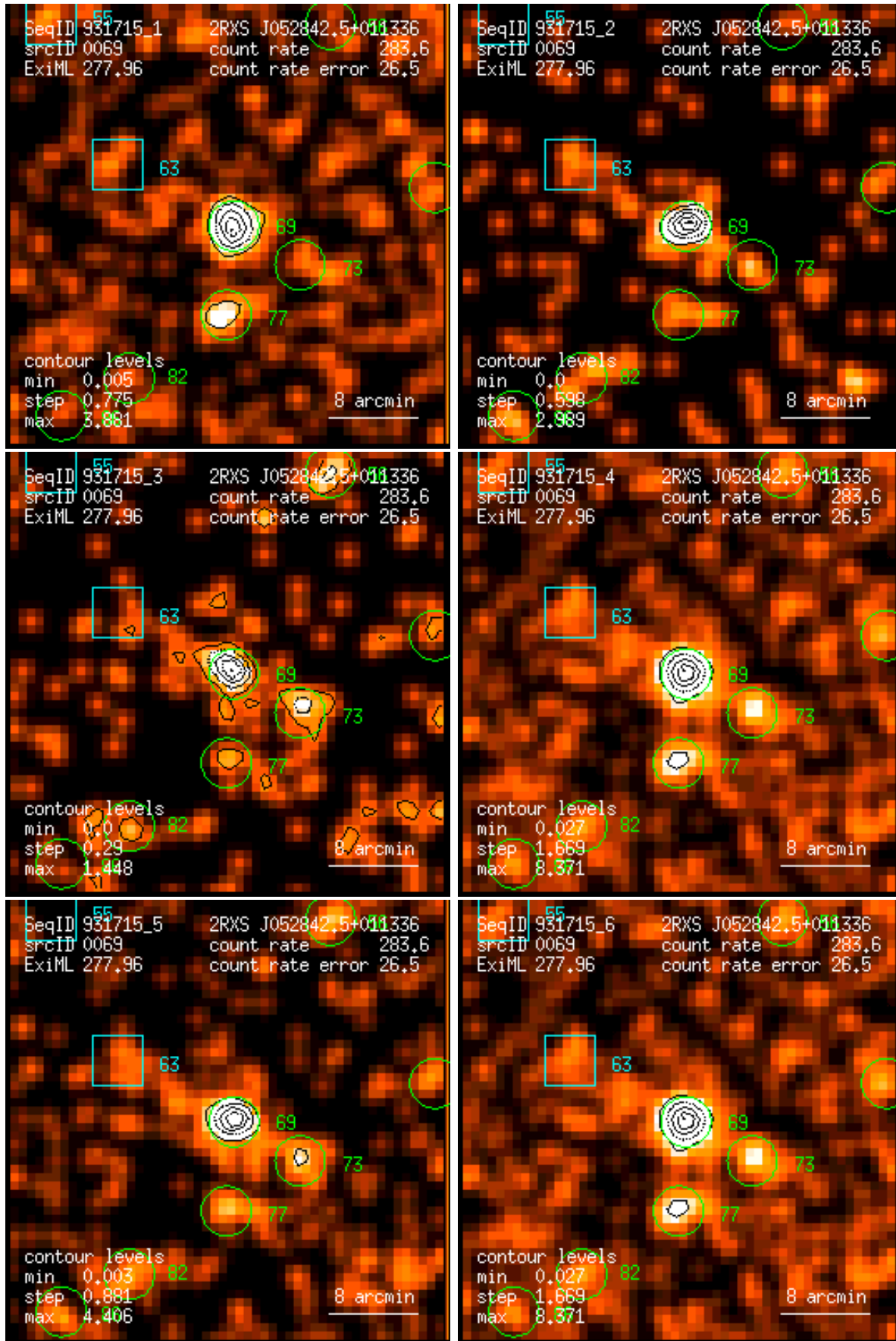
Figure 69: RASS 931715: detection 0069: band rate images, Gaussian filter: (1) PSPC channels 11 – 41, (2) 52 – 90, (3) 91 – 201, (4) 11 – 235, (5) 52 – 201, (6) 11 – 201. Broad band rates in counts/ks. Band rate contour levels in counts/ks/arcmin 2 .
