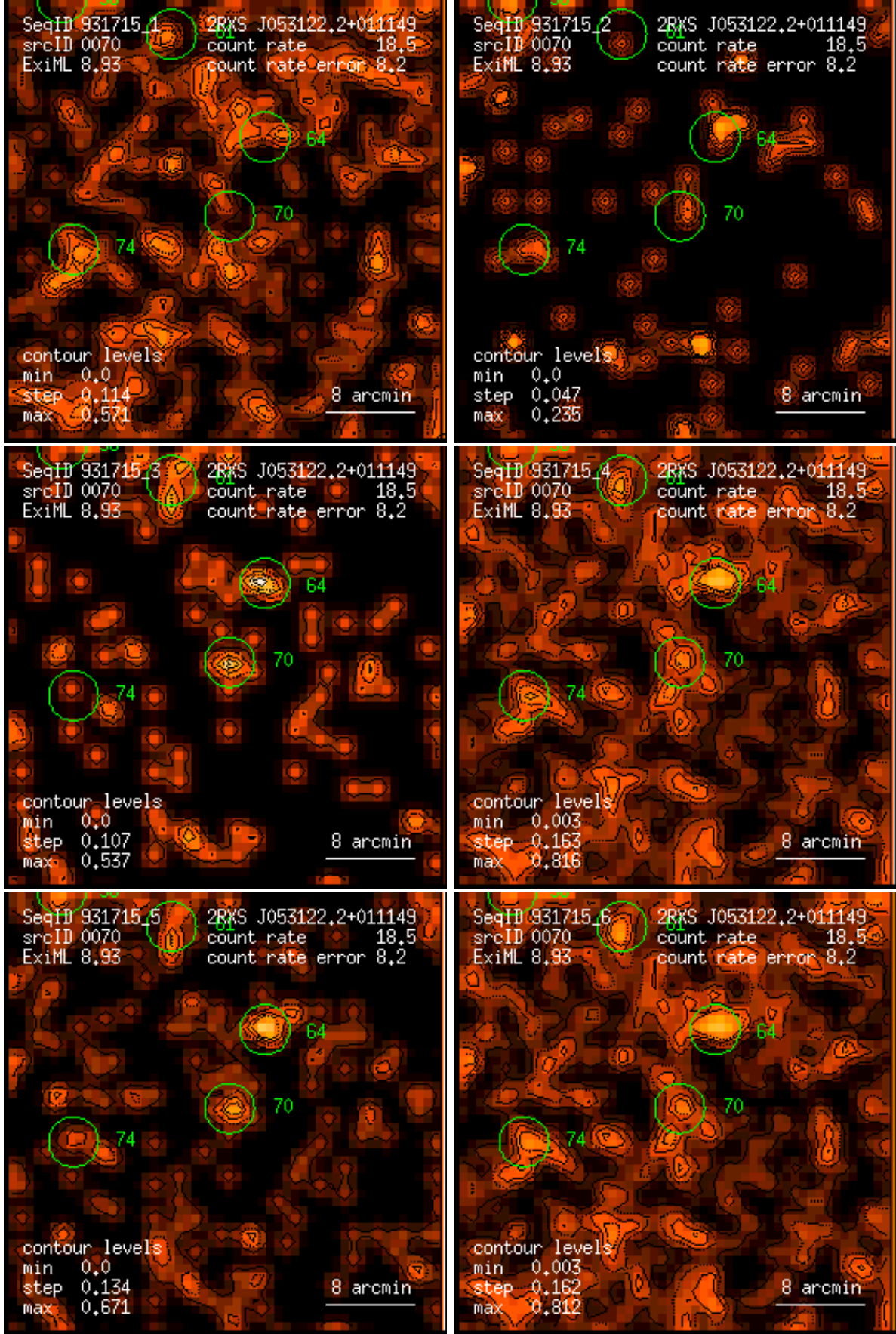
Figure 70: RASS 931715: detection 0070: band rate images, Gaussian filter: (1) PSPC channels 11 – 41, (2) 52 – 90, (3) 91 – 201, (4) 11 – 235, (5) 52 – 201, (6) 11 – 201. Broad band rates in counts/ks. Band rate contour levels in counts/ks/arcmin 2 .
