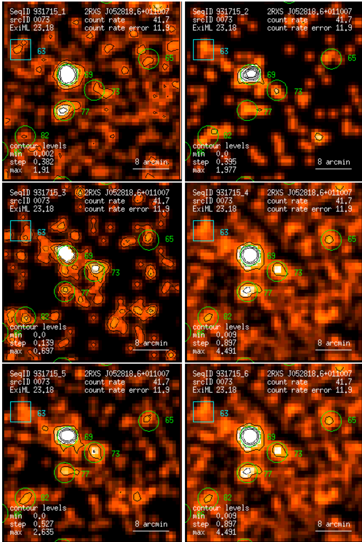
Figure 73: RASS 931715: detection 0073: band rate images, Gaussian filter: (1) PSPC channels 11 – 41, (2) 52 – 90, (3) 91 – 201, (4) 11 – 235, (5) 52 – 201, (6) 11 – 201. Broad band rates in counts/ks. Band rate contour levels in counts/ks/arcmin 2 .
