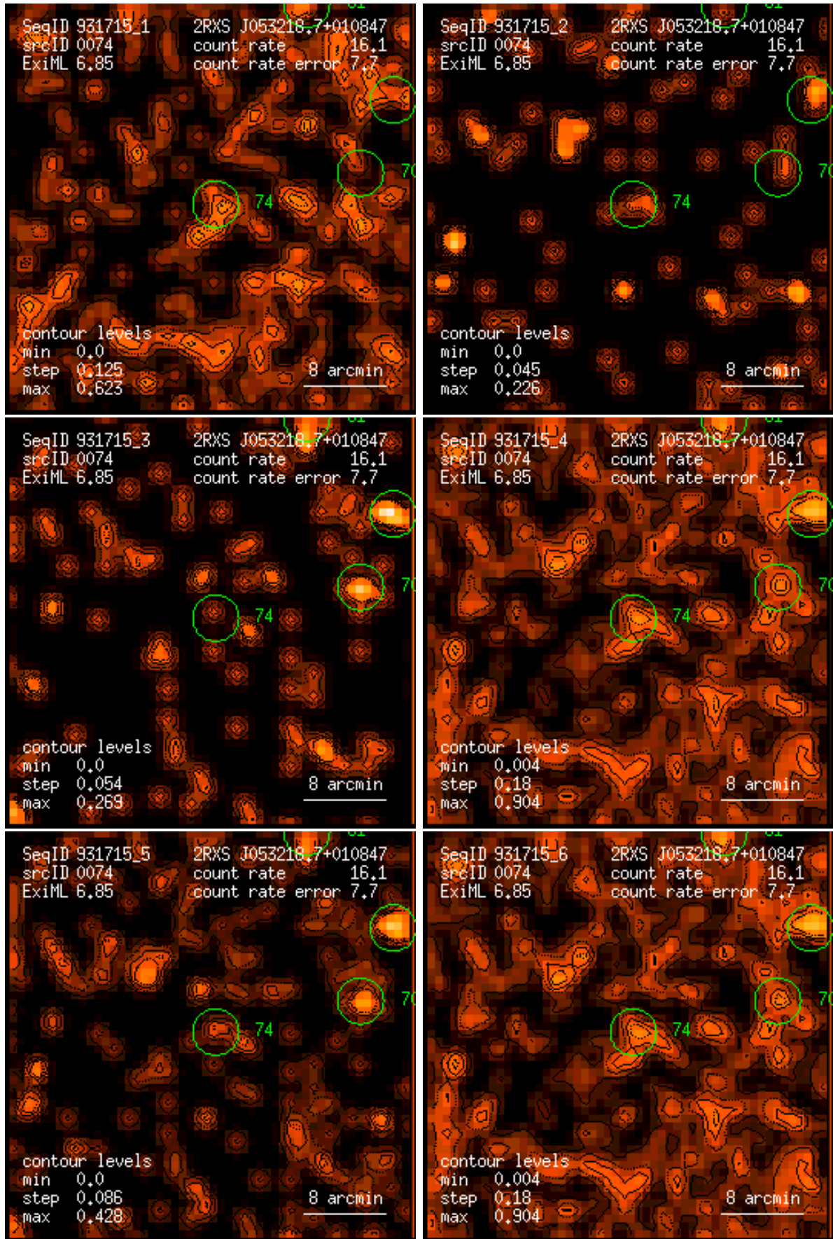
Figure 74: RASS 931715: detection 0074: band rate images, Gaussian filter: (1) PSPC channels 11 – 41, (2) 52 – 90, (3) 91 – 201, (4) 11 – 235, (5) 52 – 201, (6) 11 – 201. Broad band rates in counts/ks. Band rate contour levels in counts/ks/arcmin 2 .
