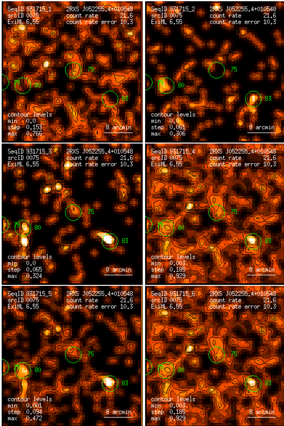
Figure 75: RASS 931715: detection 0075: band rate images, Gaussian filter: (1) PSPC channels 11 – 41, (2) 52 – 90, (3) 91 – 201, (4) 11 – 235, (5) 52 – 201, (6) 11 – 201. Broad band rates in counts/ks. Band rate contour levels in counts/ks/arcmin 2 .
