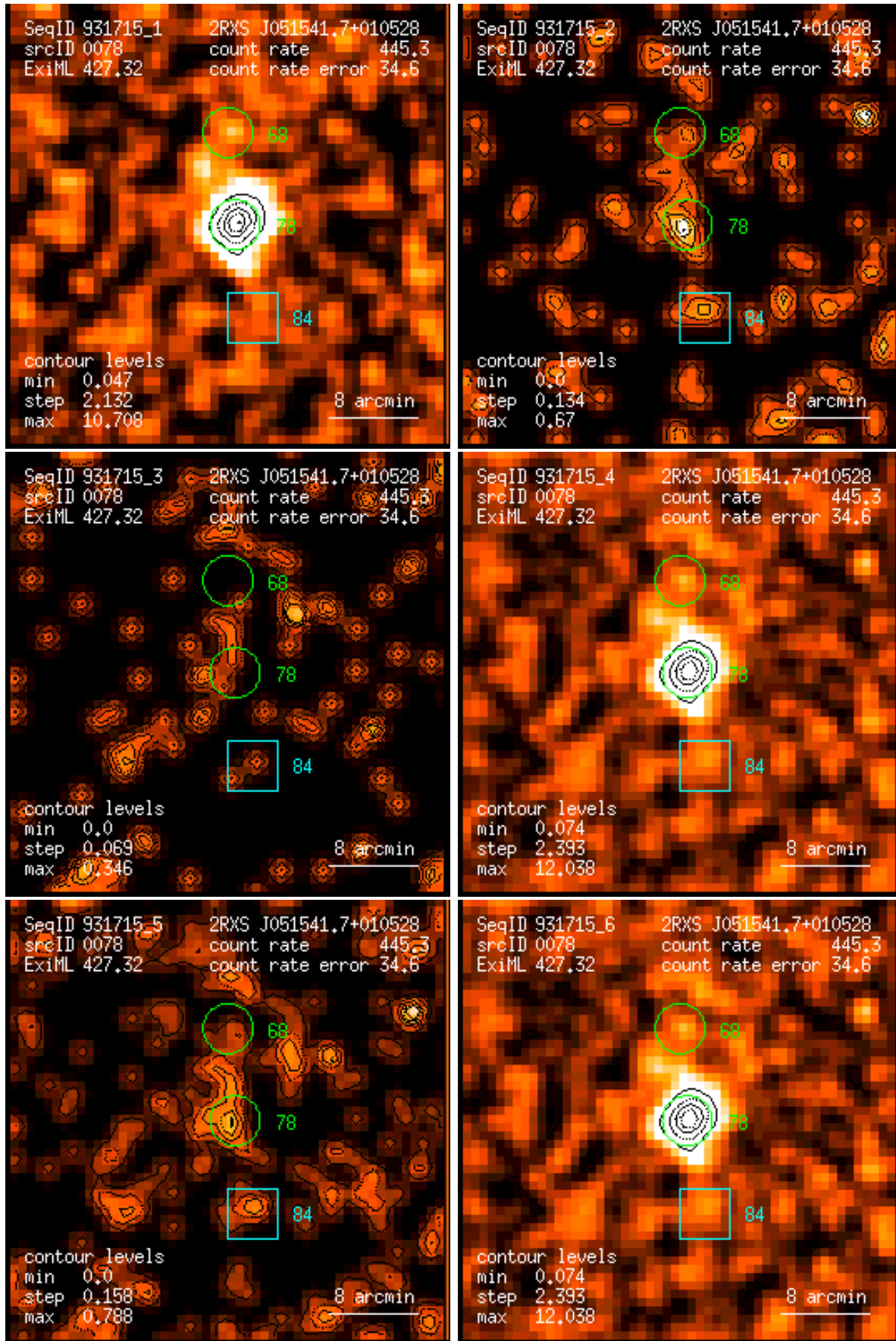
Figure 78: RASS 931715: detection 0078: band rate images, Gaussian filter: (1) PSPC channels 11 – 41, (2) 52 – 90, (3) 91 – 201, (4) 11 – 235, (5) 52 – 201, (6) 11 – 201. Broad band rates in counts/ks. Band rate contour levels in counts/ks/arcmin 2 .
