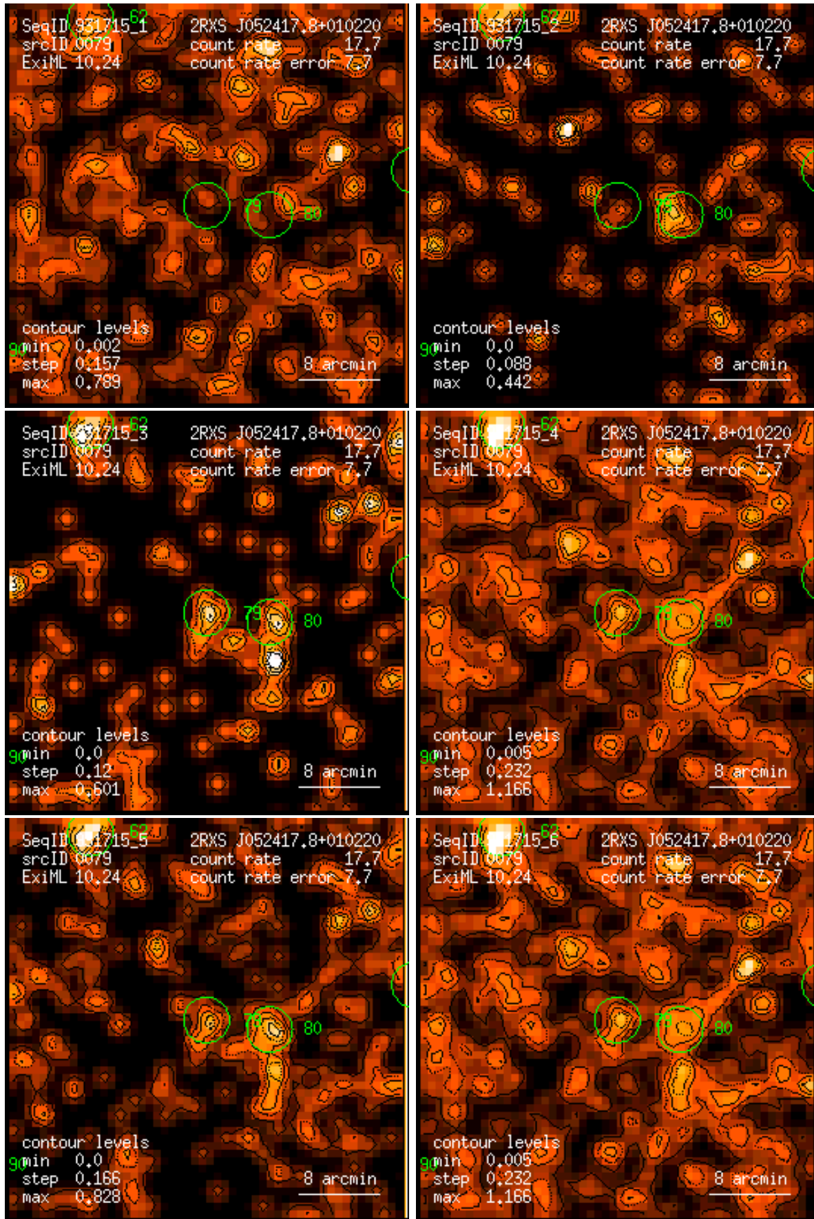
Figure 79: RASS 931715: detection 0079: band rate images, Gaussian filter: (1) PSPC channels 11 – 41, (2) 52 – 90, (3) 91 – 201, (4) 11 – 235, (5) 52 – 201, (6) 11 – 201. Broad band rates in counts/ks. Band rate contour levels in counts/ks/arcmin 2 .
