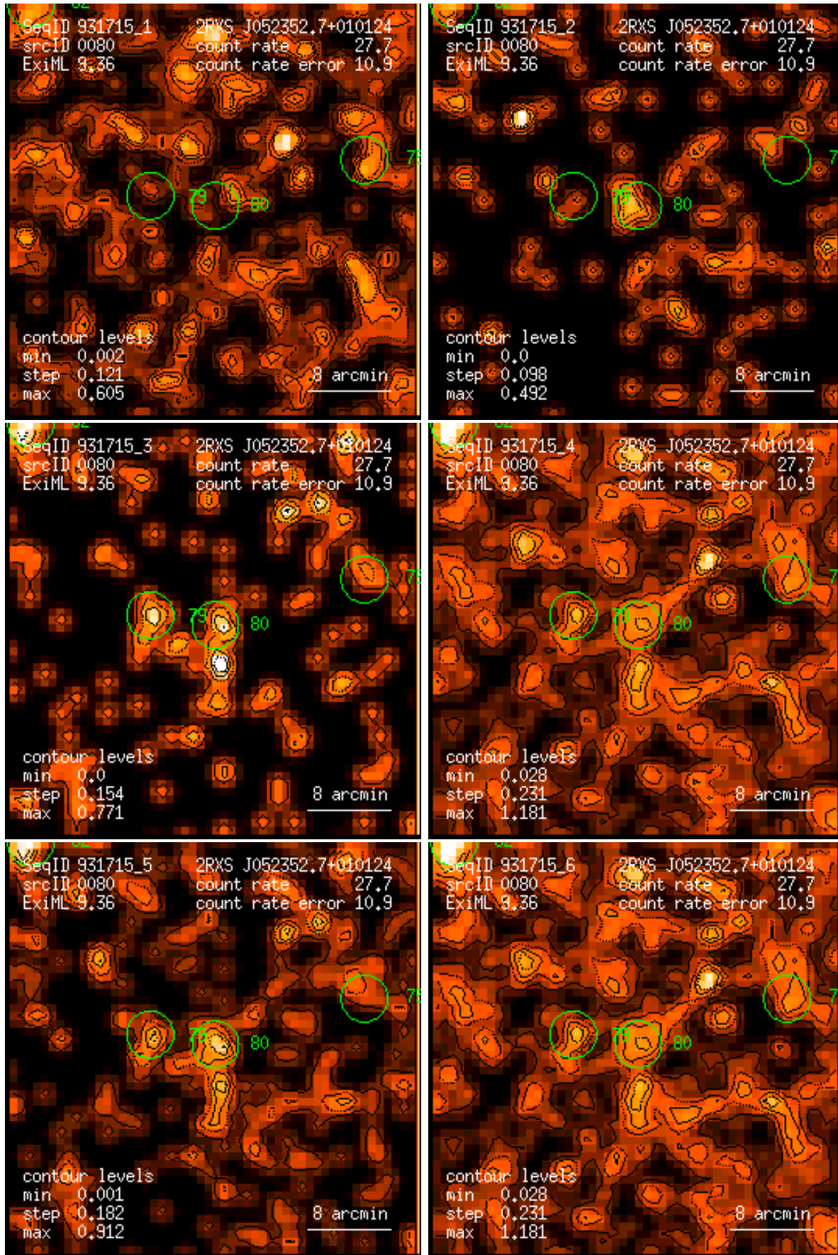
Figure 80: RASS 931715: detection 0080: band rate images, Gaussian filter: (1) PSPC channels 11 – 41, (2) 52 – 90, (3) 91 – 201, (4) 11 – 235, (5) 52 – 201, (6) 11 – 201. Broad band rates in counts/ks. Band rate contour levels in counts/ks/arcmin 2 .
