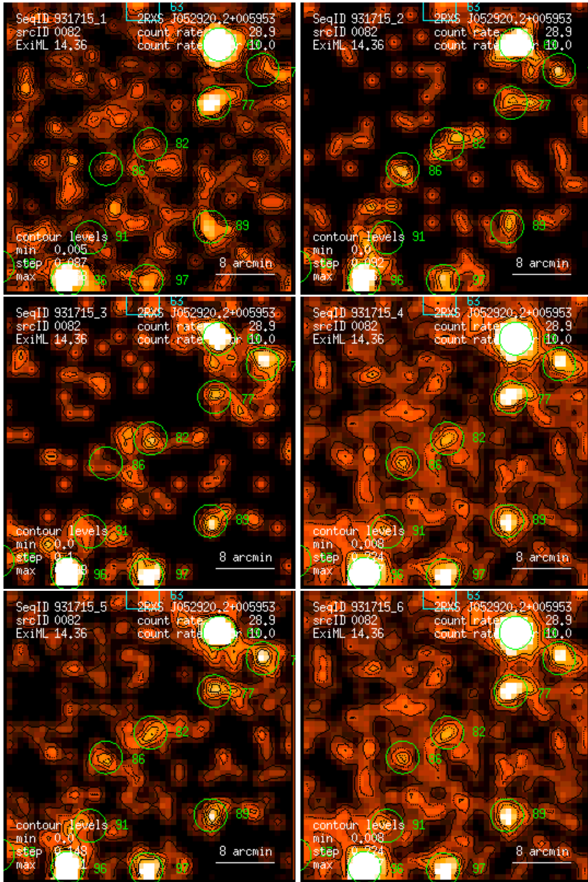
Figure 82: RASS 931715: detection 0082: band rate images, Gaussian filter: (1) PSPC channels 11 – 41, (2) 52 – 90, (3) 91 – 201, (4) 11 – 235, (5) 52 – 201, (6) 11 – 201. Broad band rates in counts/ks. Band rate contour levels in counts/ks/arcmin 2 .
