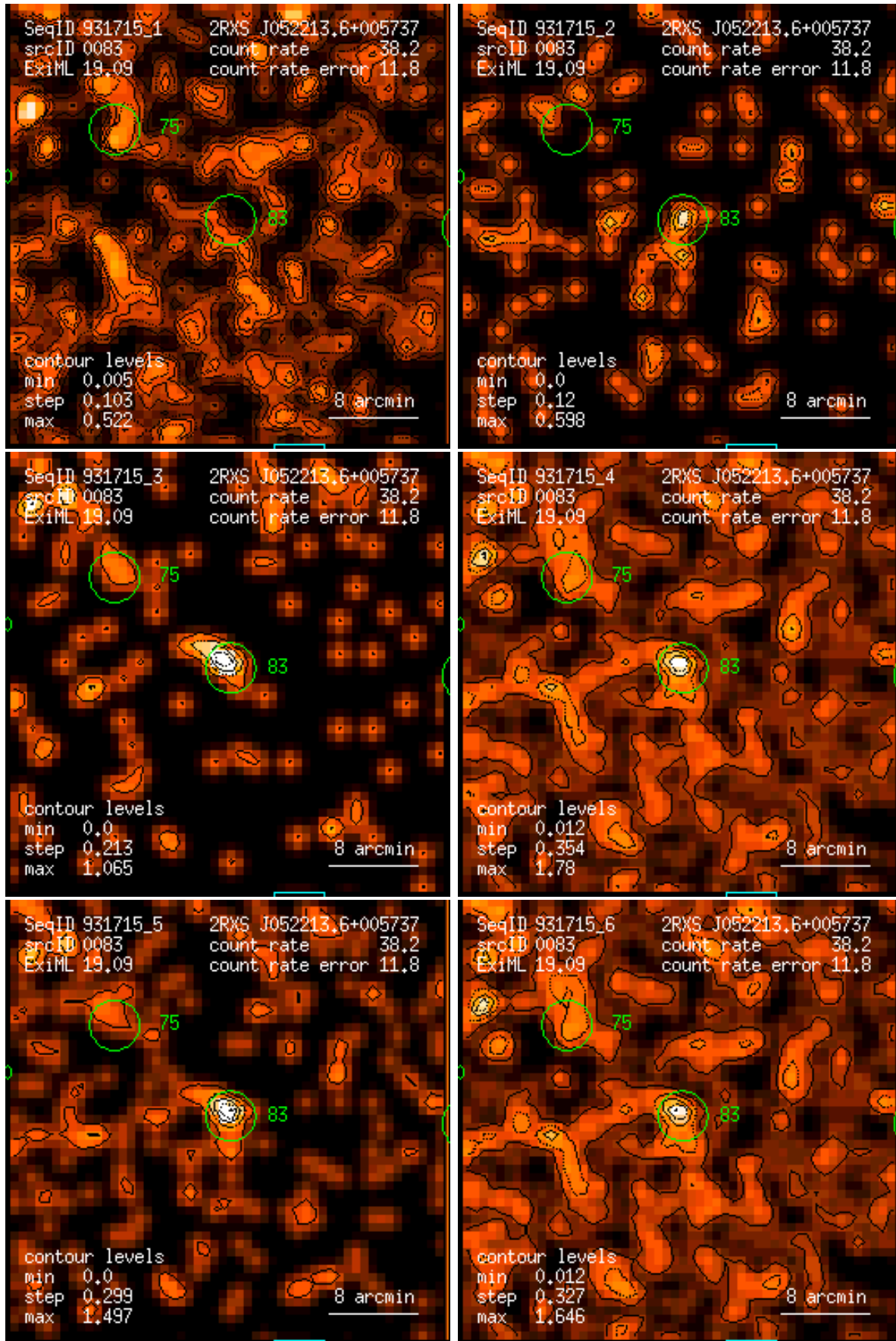
Figure 83: RASS 931715: detection 0083: band rate images, Gaussian filter: (1) PSPC channels 11 – 41, (2) 52 – 90, (3) 91 – 201, (4) 11 – 235, (5) 52 – 201, (6) 11 – 201. Broad band rates in counts/ks. Band rate contour levels in counts/ks/arcmin 2 .
