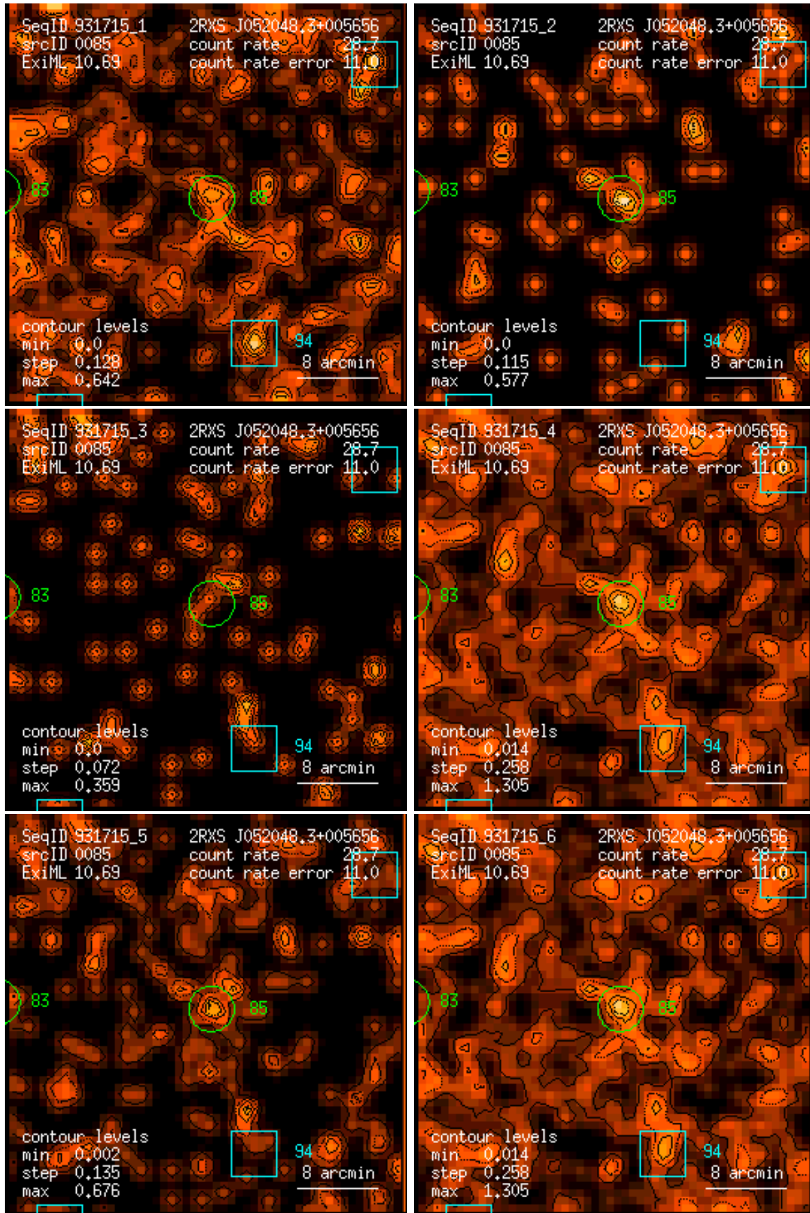
Figure 85: RASS 931715: detection 0085: band rate images, Gaussian filter: (1) PSPC channels 11 – 41, (2) 52 – 90, (3) 91 – 201, (4) 11 – 235, (5) 52 – 201, (6) 11 – 201. Broad band rates in counts/ks. Band rate contour levels in counts/ks/arcmin 2 .
