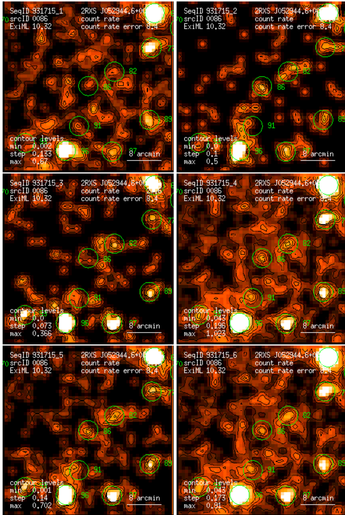
Figure 86: RASS 931715: detection 0086: band rate images, Gaussian filter: (1) PSPC channels 11 – 41, (2) 52 – 90, (3) 91 – 201, (4) 11 – 235, (5) 52 – 201, (6) 11 – 201. Broad band rates in counts/ks. Band rate contour levels in counts/ks/arcmin 2 .
