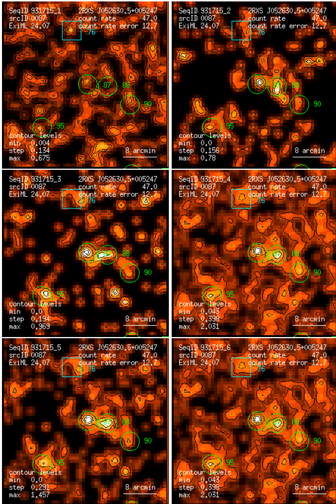
Figure 87: RASS 931715: detection 0087: band rate images, Gaussian filter: (1) PSPC channels 11 – 41, (2) 52 – 90, (3) 91 – 201, (4) 11 – 235, (5) 52 – 201, (6) 11 – 201. Broad band rates in counts/ks. Band rate contour levels in counts/ks/arcmin 2 .
