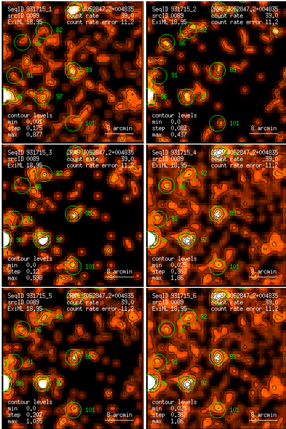
Figure 89: RASS 931715: detection 0089: band rate images, Gaussian filter: (1) PSPC channels 11 – 41, (2) 52 – 90, (3) 91 – 201, (4) 11 – 235, (5) 52 – 201, (6) 11 – 201. Broad band rates in counts/ks. Band rate contour levels in counts/ks/arcmin 2 .
