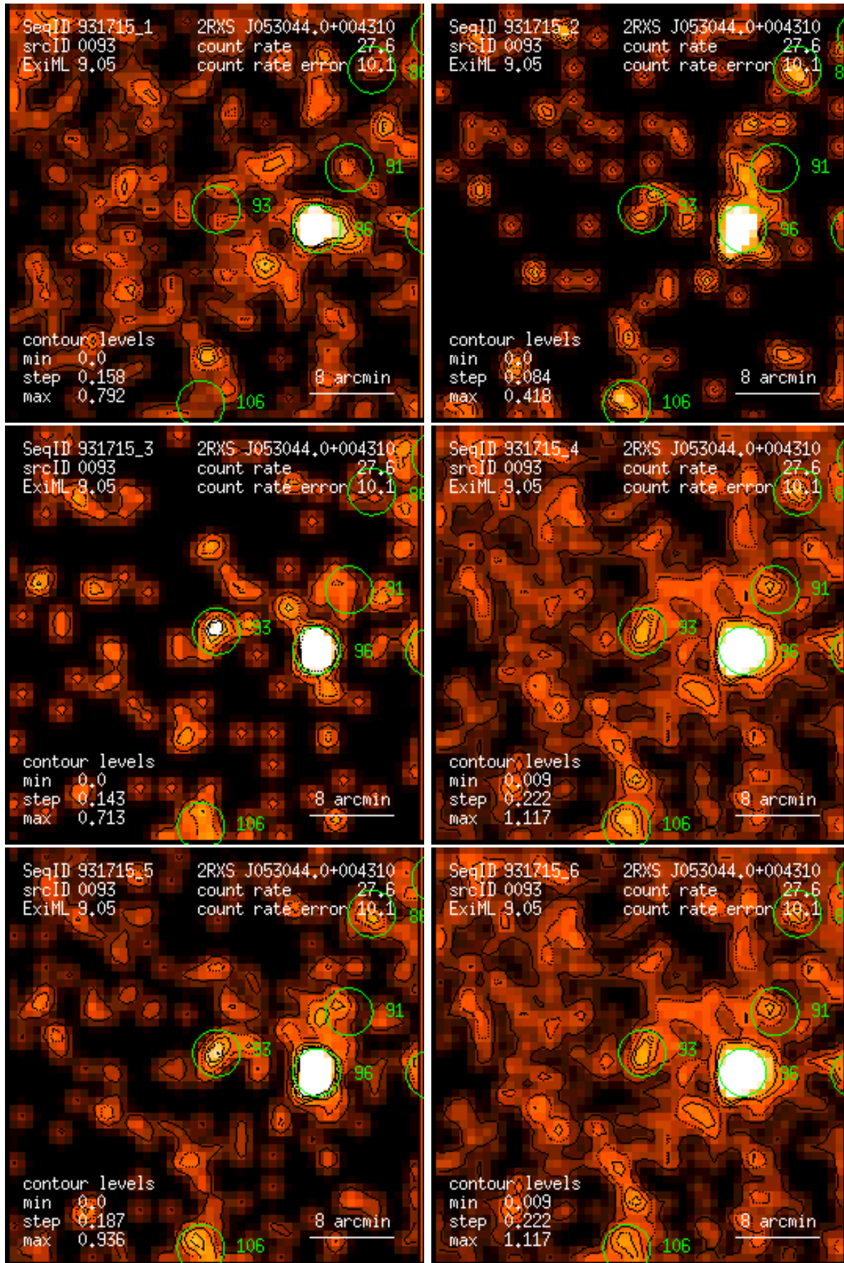
Figure 93: RASS 931715: detection 0093: band rate images, Gaussian filter: (1) PSPC channels 11 – 41, (2) 52 – 90, (3) 91 – 201, (4) 11 – 235, (5) 52 – 201, (6) 11 – 201. Broad band rates in counts/ks. Band rate contour levels in counts/ks/arcmin 2 .
