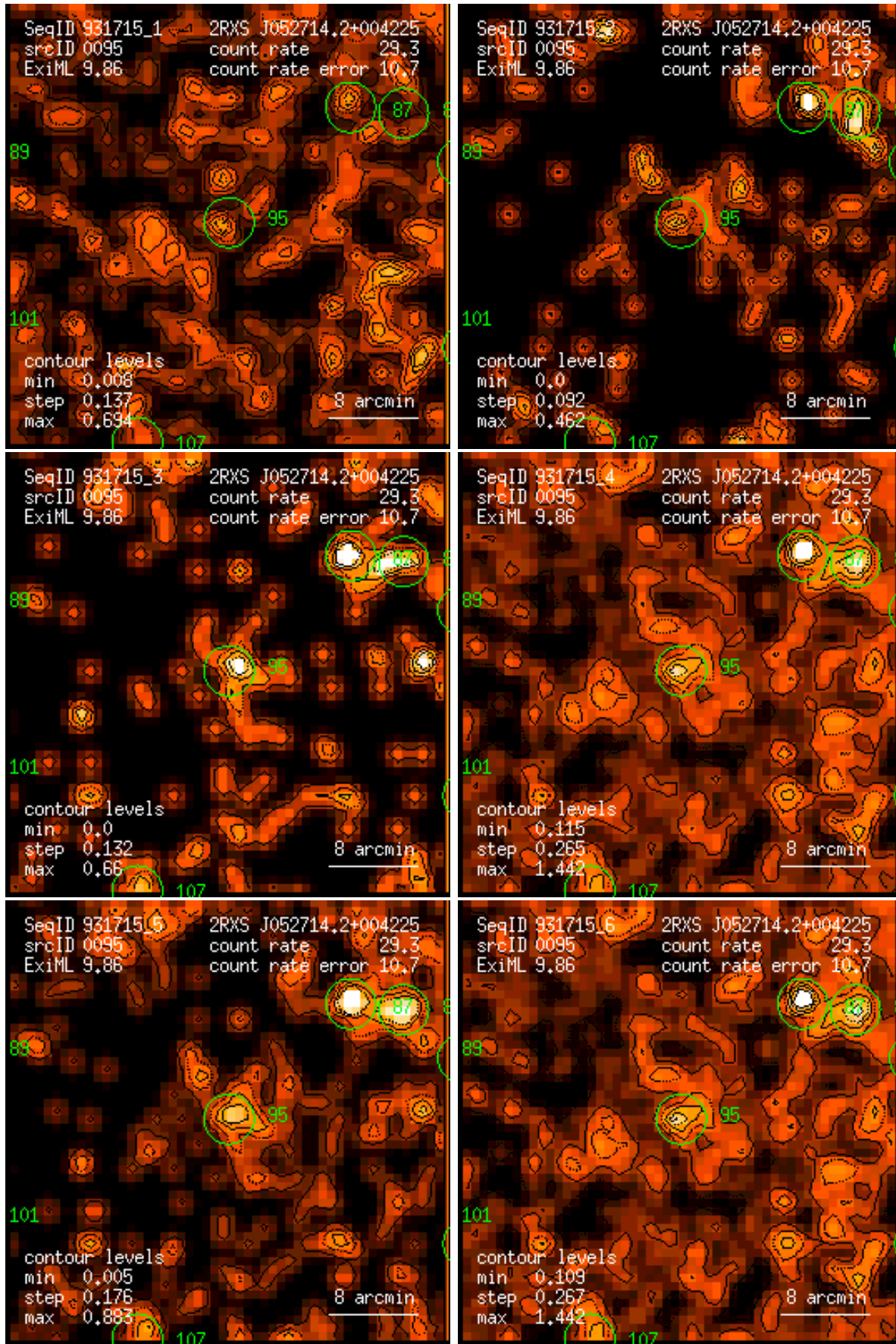
Figure 95: RASS 931715: detection 0095: band rate images, Gaussian filter: (1) PSPC channels 11 – 41, (2) 52 – 90, (3) 91 – 201, (4) 11 – 235, (5) 52 – 201, (6) 11 – 201. Broad band rates in counts/ks. Band rate contour levels in counts/ks/arcmin 2 .
