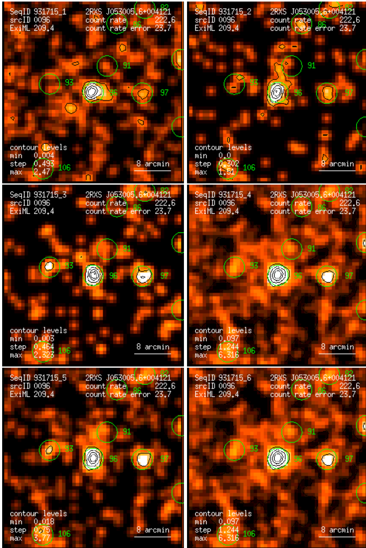
Figure 96: RASS 931715: detection 0096: band rate images, Gaussian filter: (1) PSPC channels 11 – 41, (2) 52 – 90, (3) 91 – 201, (4) 11 – 235, (5) 52 – 201, (6) 11 – 201. Broad band rates in counts/ks. Band rate contour levels in counts/ks/arcmin 2 .
