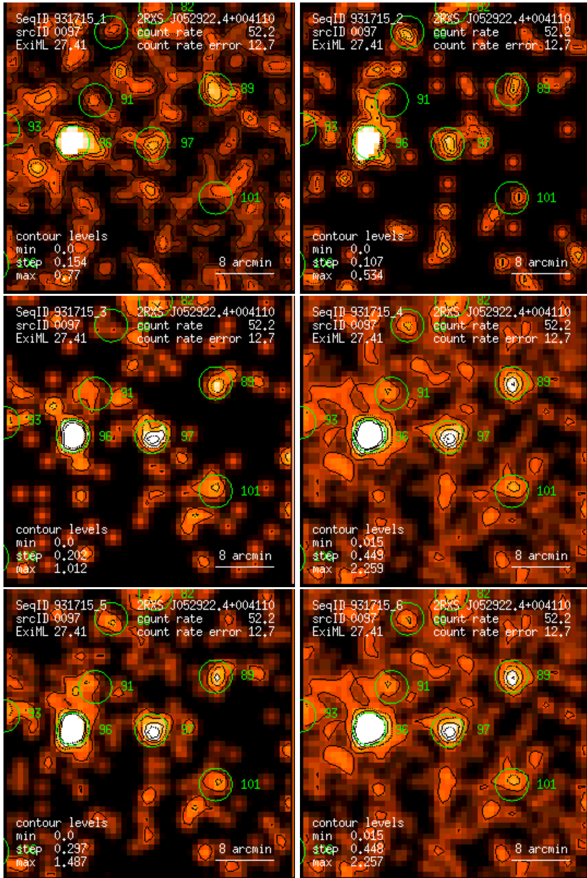
Figure 97: RASS 931715: detection 0097: band rate images, Gaussian filter: (1) PSPC channels 11 – 41, (2) 52 – 90, (3) 91 – 201, (4) 11 – 235, (5) 52 – 201, (6) 11 – 201. Broad band rates in counts/ks. Band rate contour levels in counts/ks/arcmin 2 .
