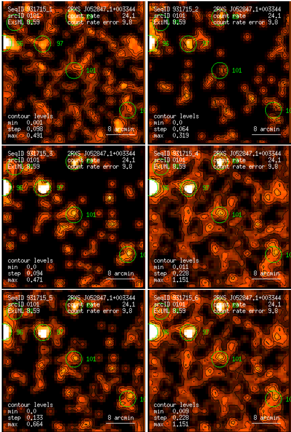
Figure 101: RASS 931715: detection 0101: band rate images, Gaussian filter: (1) PSPC channels 11 – 41, (2) 52 – 90, (3) 91 – 201, (4) 11 – 235, (5) 52 – 201, (6) 11 – 201. Broad band rates in counts/ks. Band rate contour levels in counts/ks/arcmin 2 .
