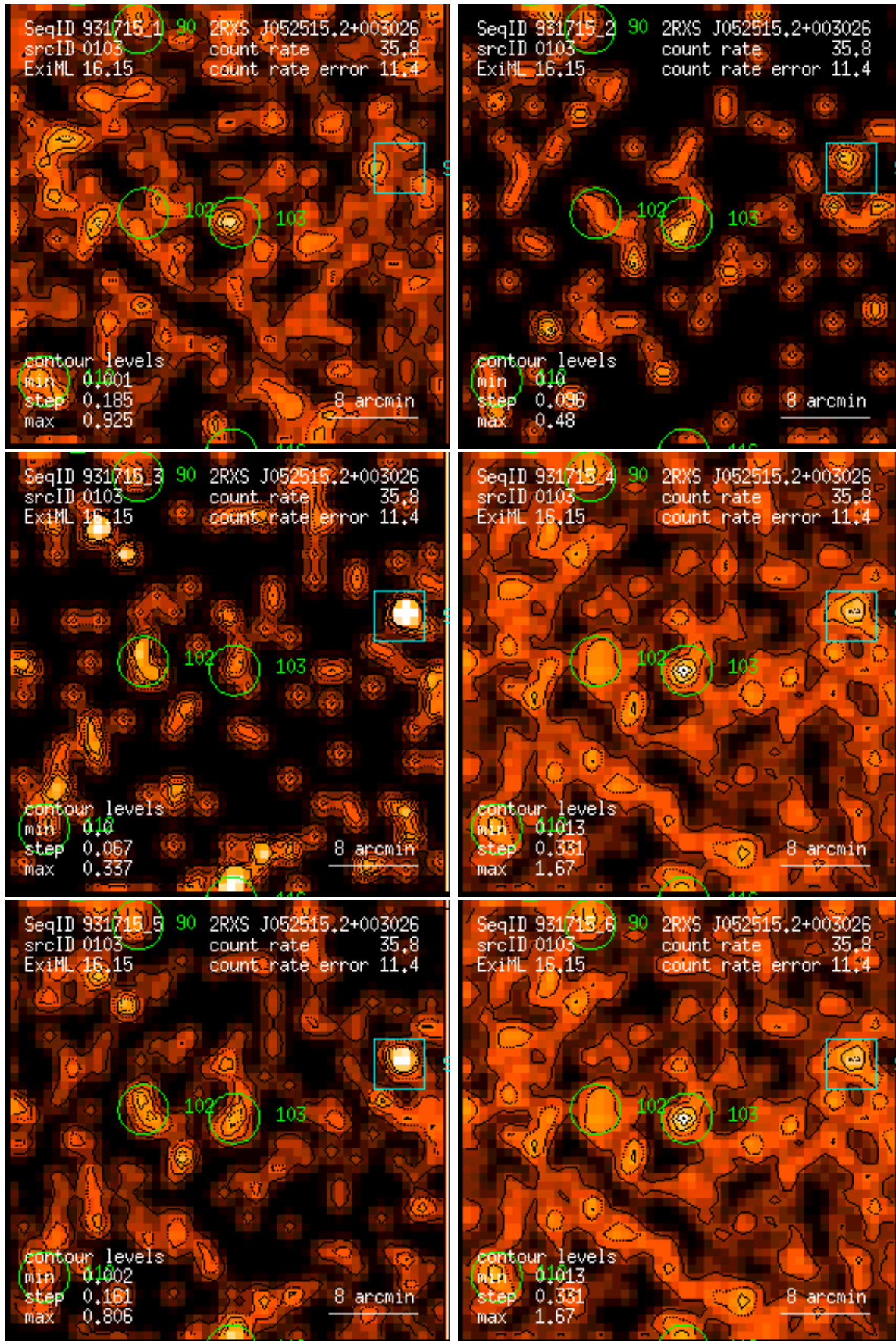
Figure 103: RASS 931715: detection 0103: band rate images, Gaussian filter: (1) PSPC channels 11 – 41, (2) 52 – 90, (3) 91 – 201, (4) 11 – 235, (5) 52 – 201, (6) 11 – 201. Broad band rates in counts/ks. Band rate contour levels in counts/ks/arcmin 2 .
