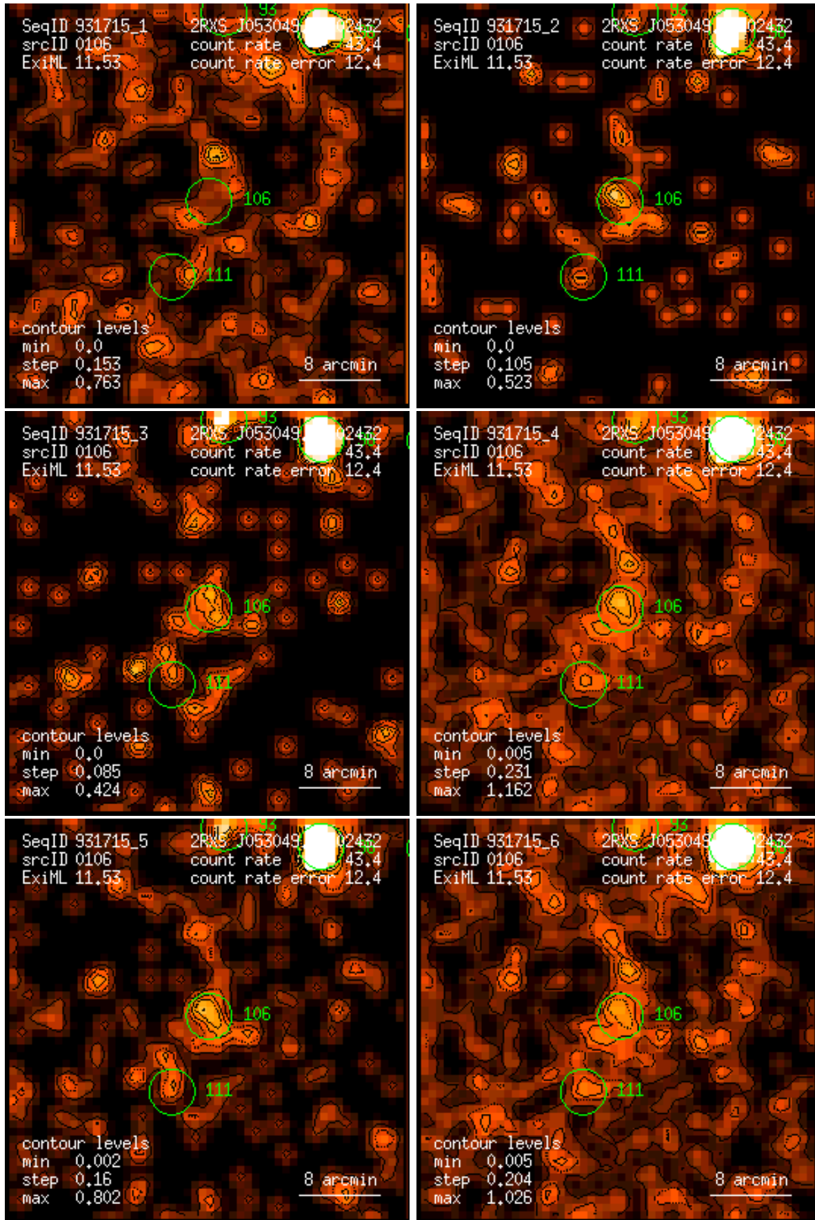
Figure 106: RASS 931715: detection 0106: band rate images, Gaussian filter: (1) PSPC channels 11 – 41, (2) 52 – 90, (3) 91 – 201, (4) 11 – 235, (5) 52 – 201, (6) 11 – 201. Broad band rates in counts/ks. Band rate contour levels in counts/ks/arcmin 2 .
