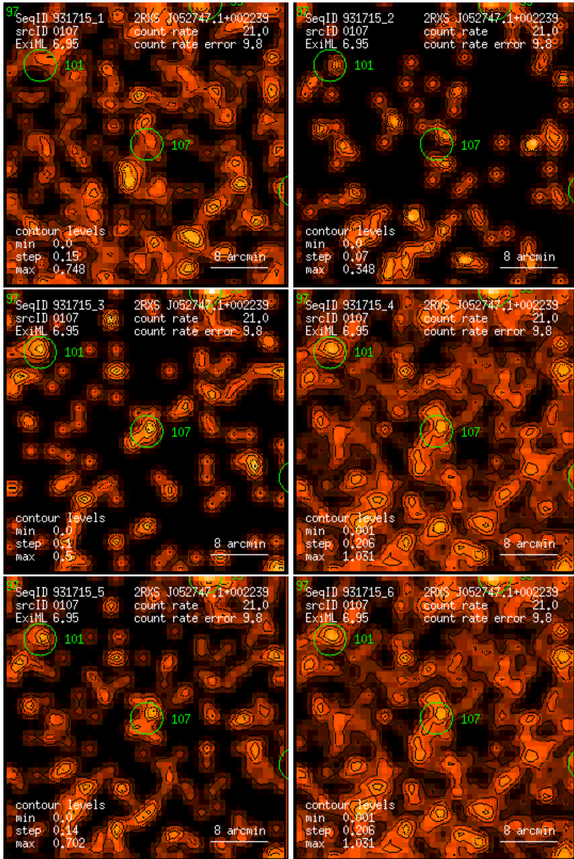
Figure 107: RASS 931715: detection 0107: band rate images, Gaussian filter: (1) PSPC channels 11 – 41, (2) 52 – 90, (3) 91 – 201, (4) 11 – 235, (5) 52 – 201, (6) 11 – 201. Broad band rates in counts/ks. Band rate contour levels in counts/ks/arcmin 2 .
