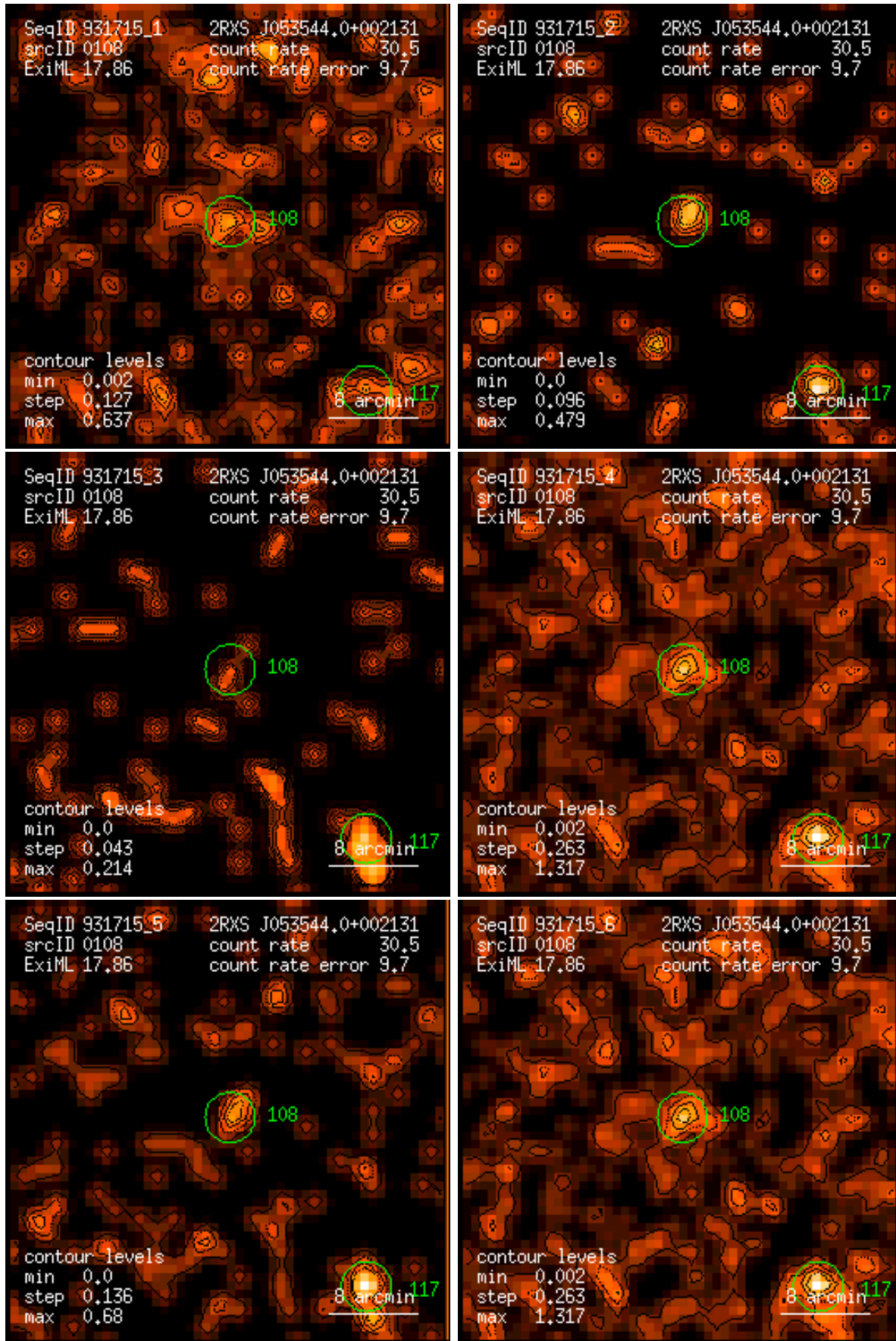
Figure 108: RASS 931715: detection 0108: band rate images, Gaussian filter: (1) PSPC channels 11 – 41, (2) 52 – 90, (3) 91 – 201, (4) 11 – 235, (5) 52 – 201, (6) 11 – 201. Broad band rates in counts/ks. Band rate contour levels in counts/ks/arcmin 2 .
