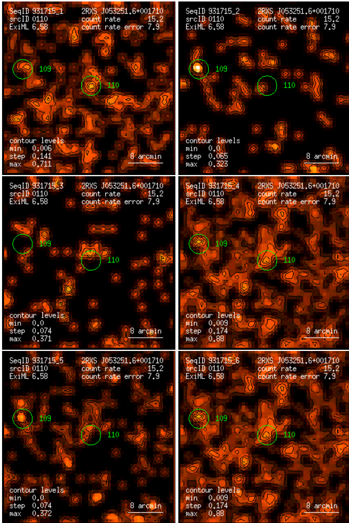
Figure 110: RASS 931715: detection 0110: band rate images, Gaussian filter: (1) PSPC channels 11 – 41, (2) 52 – 90, (3) 91 – 201, (4) 11 – 235, (5) 52 – 201, (6) 11 – 201. Broad band rates in counts/ks. Band rate contour levels in counts/ks/arcmin 2 .
