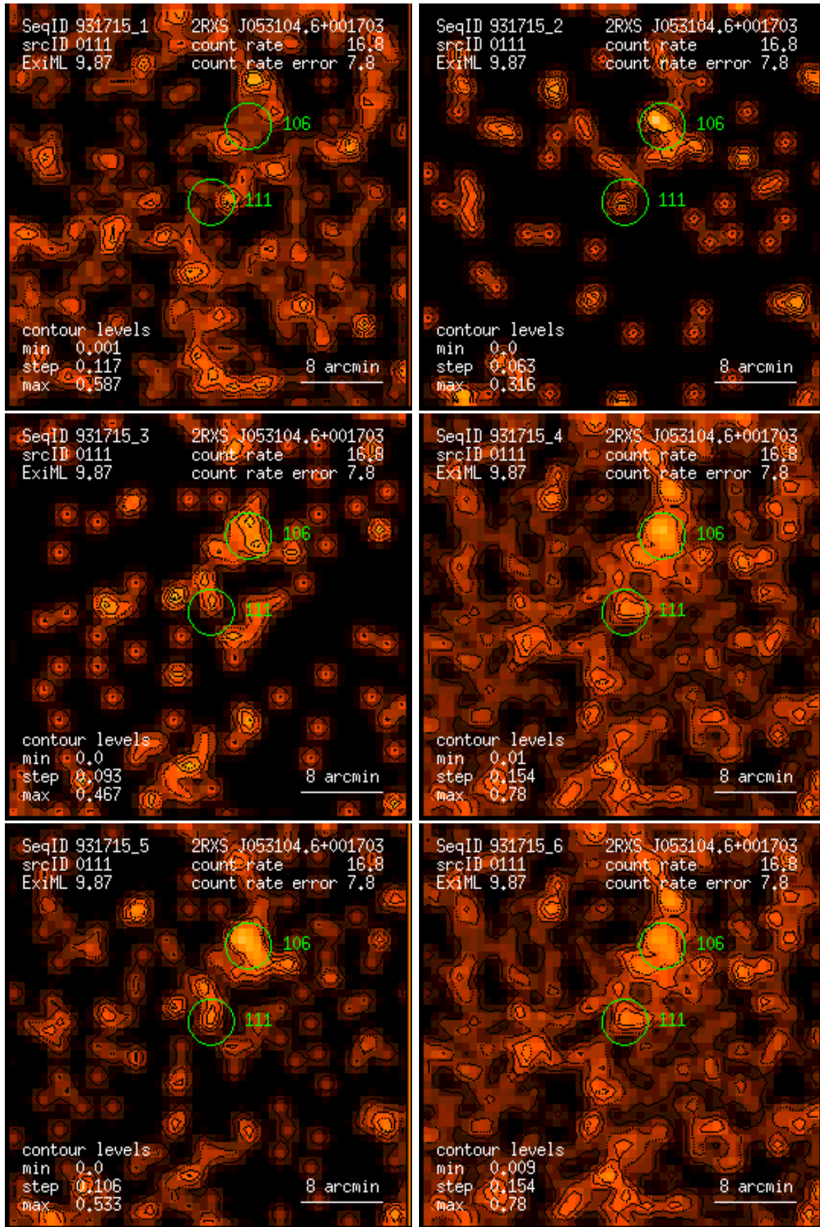
Figure 111: RASS 931715: detection 0111: band rate images, Gaussian filter: (1) PSPC channels 11 – 41, (2) 52 – 90, (3) 91 – 201, (4) 11 – 235, (5) 52 – 201, (6) 11 – 201. Broad band rates in counts/ks. Band rate contour levels in counts/ks/arcmin 2 .
