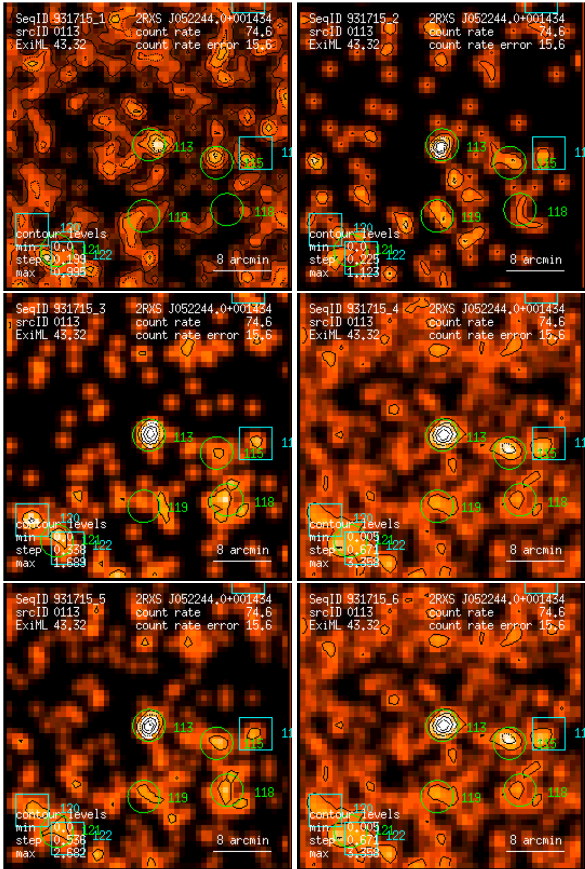
Figure 113: RASS 931715: detection 0113: band rate images, Gaussian filter: (1) PSPC channels 11 – 41, (2) 52 – 90, (3) 91 – 201, (4) 11 – 235, (5) 52 – 201, (6) 11 – 201. Broad band rates in counts/ks. Band rate contour levels in counts/ks/arcmin 2 .
