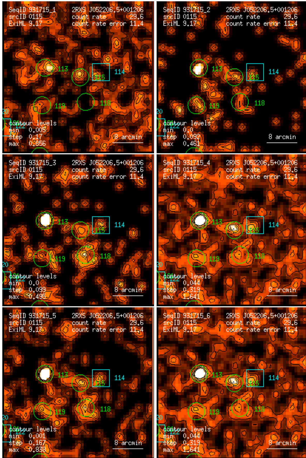
Figure 115: RASS 931715: detection 0115: band rate images, Gaussian filter: (1) PSPC channels 11 – 41, (2) 52 – 90, (3) 91 – 201, (4) 11 – 235, (5) 52 – 201, (6) 11 – 201. Broad band rates in counts/ks. Band rate contour levels in counts/ks/arcmin 2 .
