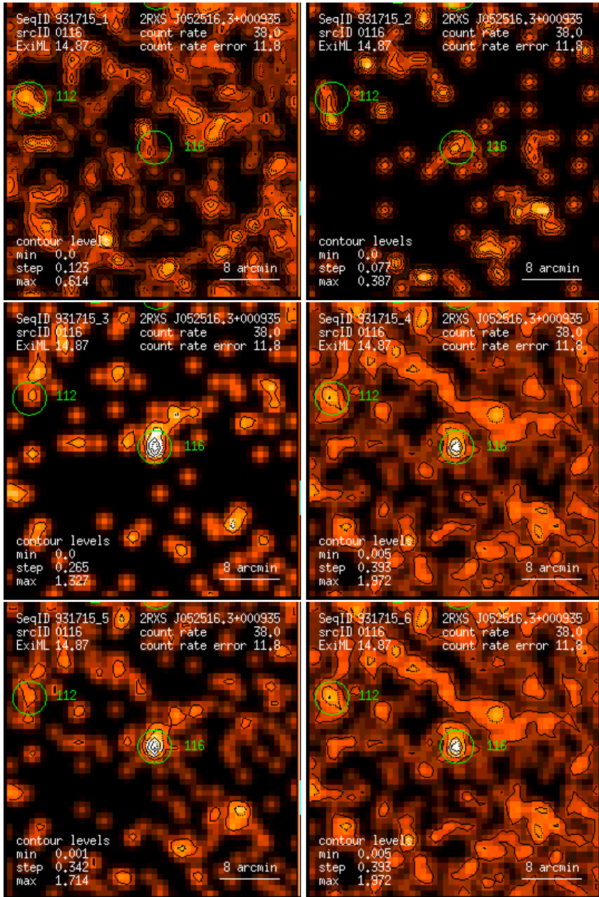
Figure 116: RASS 931715: detection 0116: band rate images, Gaussian filter: (1) PSPC channels 11 – 41, (2) 52 – 90, (3) 91 – 201, (4) 11 – 235, (5) 52 – 201, (6) 11 – 201. Broad band rates in counts/ks. Band rate contour levels in counts/ks/arcmin 2 .
