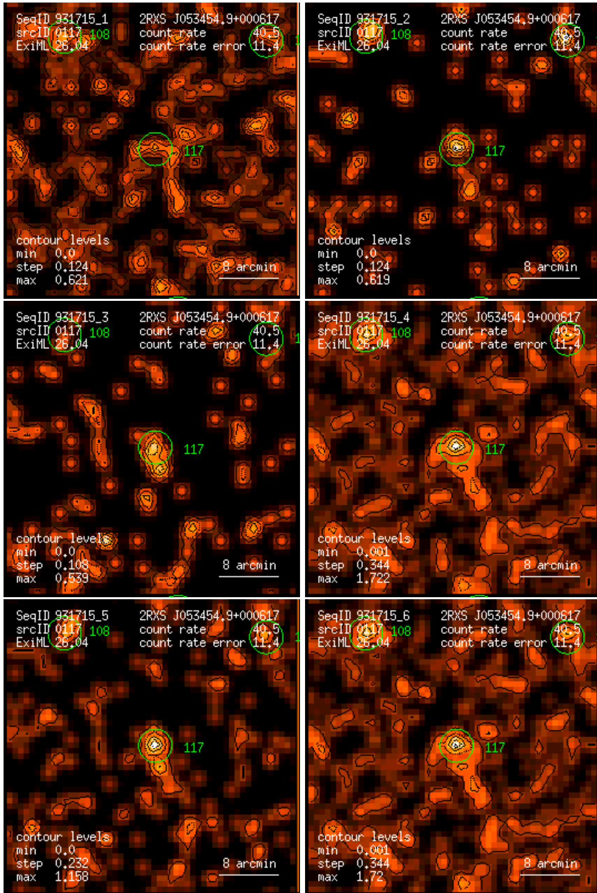
Figure 117: RASS 931715: detection 0117: band rate images, Gaussian filter: (1) PSPC channels 11 – 41, (2) 52 – 90, (3) 91 – 201, (4) 11 – 235, (5) 52 – 201, (6) 11 – 201. Broad band rates in counts/ks. Band rate contour levels in counts/ks/arcmin 2 .
