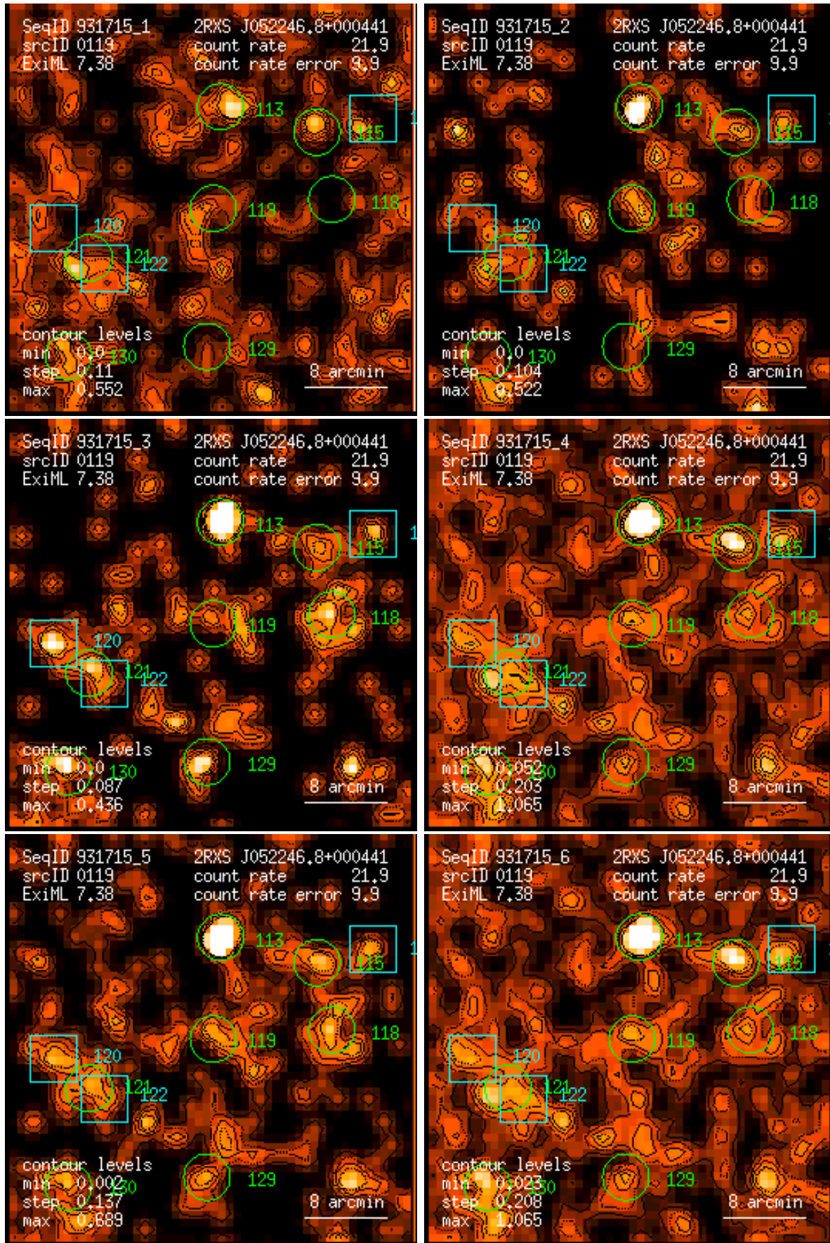
Figure 119: RASS 931715: detection 0119: band rate images, Gaussian filter: (1) PSPC channels 11 – 41, (2) 52 – 90, (3) 91 – 201, (4) 11 – 235, (5) 52 – 201, (6) 11 – 201. Broad band rates in counts/ks. Band rate contour levels in counts/ks/arcmin 2 .
