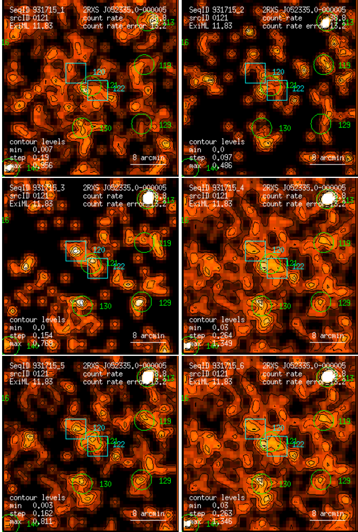
Figure 121: RASS 931715: detection 0121: band rate images, Gaussian filter: (1) PSPC channels 11 – 41, (2) 52 – 90, (3) 91 – 201, (4) 11 – 235, (5) 52 – 201, (6) 11 – 201. Broad band rates in counts/ks. Band rate contour levels in counts/ks/arcmin 2 .
