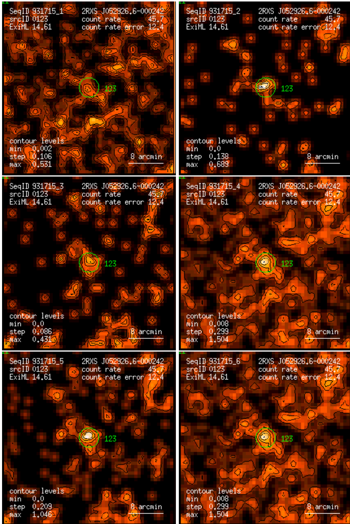
Figure 123: RASS 931715: detection 0123: band rate images, Gaussian filter: (1) PSPC channels 11 – 41, (2) 52 – 90, (3) 91 – 201, (4) 11 – 235, (5) 52 – 201, (6) 11 – 201. Broad band rates in counts/ks. Band rate contour levels in counts/ks/arcmin 2 .
