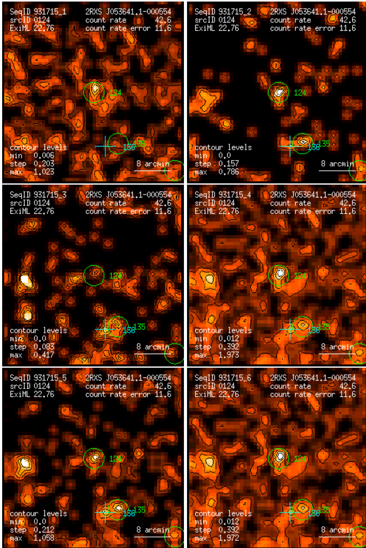
Figure 124: RASS 931715: detection 0124: band rate images, Gaussian filter: (1) PSPC channels 11 – 41, (2) 52 – 90, (3) 91 – 201, (4) 11 – 235, (5) 52 – 201, (6) 11 – 201. Broad band rates in counts/ks. Band rate contour levels in counts/ks/arcmin 2 .
