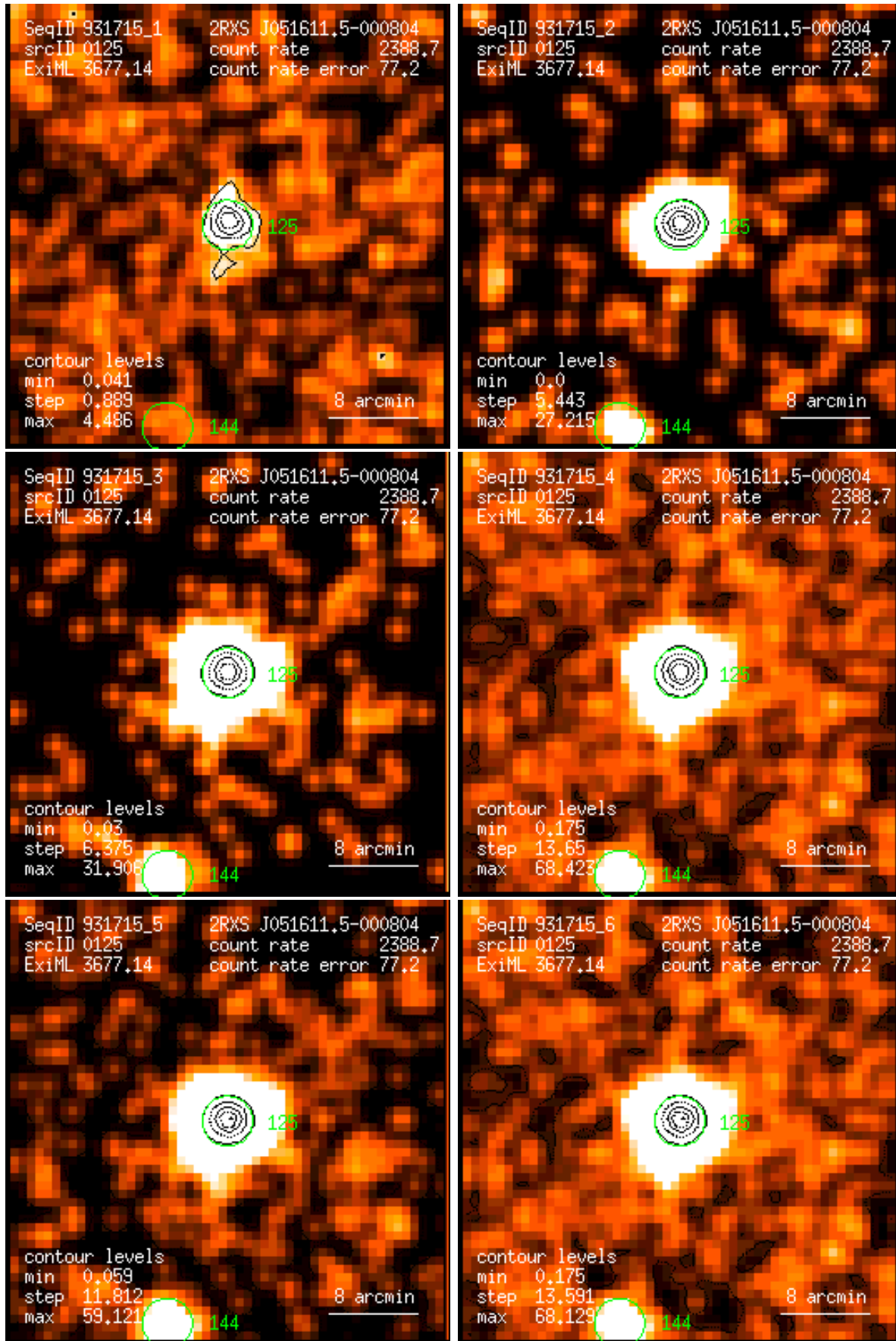
Figure 125: RASS 931715: detection 0125: band rate images, Gaussian filter: (1) PSPC channels 11 – 41, (2) 52 – 90, (3) 91 – 201, (4) 11 – 235, (5) 52 – 201, (6) 11 – 201. Broad band rates in counts/ks. Band rate contour levels in counts/ks/arcmin 2 .
