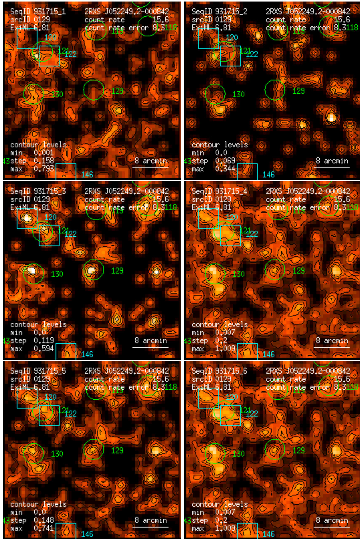
Figure 129: RASS 931715: detection 0129: band rate images, Gaussian filter: (1) PSPC channels 11 – 41, (2) 52 – 90, (3) 91 – 201, (4) 11 – 235, (5) 52 – 201, (6) 11 – 201. Broad band rates in counts/ks. Band rate contour levels in counts/ks/arcmin 2 .
