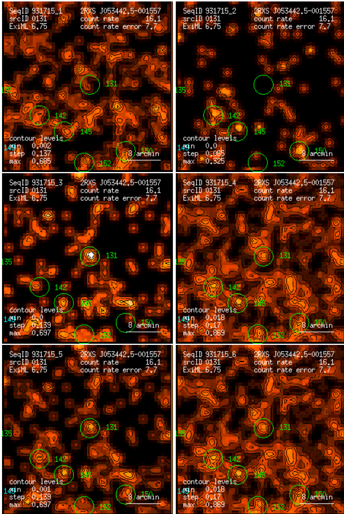
Figure 131: RASS 931715: detection 0131: band rate images, Gaussian filter: (1) PSPC channels 11 – 41, (2) 52 – 90, (3) 91 – 201, (4) 11 – 235, (5) 52 – 201, (6) 11 – 201. Broad band rates in counts/ks. Band rate contour levels in counts/ks/arcmin 2 .
