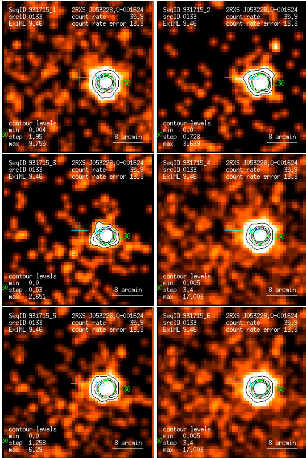
Figure 133: RASS 931715: detection 0133: band rate images, Gaussian filter: (1) PSPC channels 11 – 41, (2) 52 – 90, (3) 91 – 201, (4) 11 – 235, (5) 52 – 201, (6) 11 – 201. Broad band rates in counts/ks. Band rate contour levels in counts/ks/arcmin 2 .
