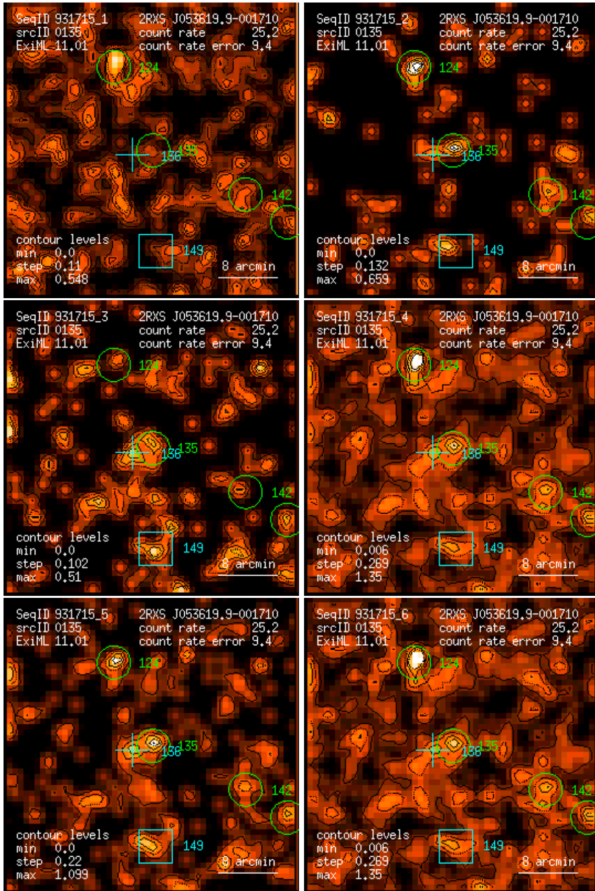
Figure 135: RASS 931715: detection 0135: band rate images, Gaussian filter: (1) PSPC channels 11 – 41, (2) 52 – 90, (3) 91 – 201, (4) 11 – 235, (5) 52 – 201, (6) 11 – 201. Broad band rates in counts/ks. Band rate contour levels in counts/ks/arcmin 2 .
