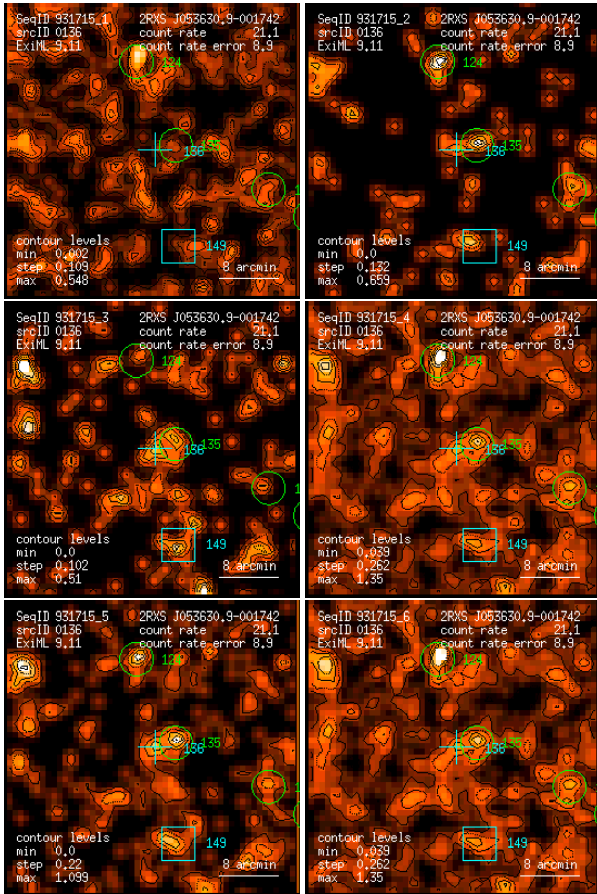
Figure 136: RASS 931715: detection 0136: band rate images, Gaussian filter: (1) PSPC channels 11 – 41, (2) 52 – 90, (3) 91 – 201, (4) 11 – 235, (5) 52 – 201, (6) 11 – 201. Broad band rates in counts/ks. Band rate contour levels in counts/ks/arcmin 2 .
