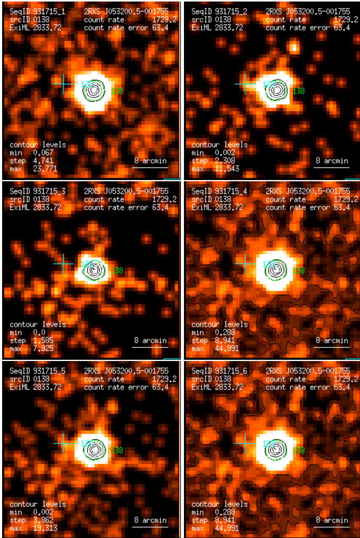
Figure 138: RASS 931715: detection 0138: band rate images, Gaussian filter: (1) PSPC channels 11 – 41, (2) 52 – 90, (3) 91 – 201, (4) 11 – 235, (5) 52 – 201, (6) 11 – 201. Broad band rates in counts/ks. Band rate contour levels in counts/ks/arcmin 2 .
