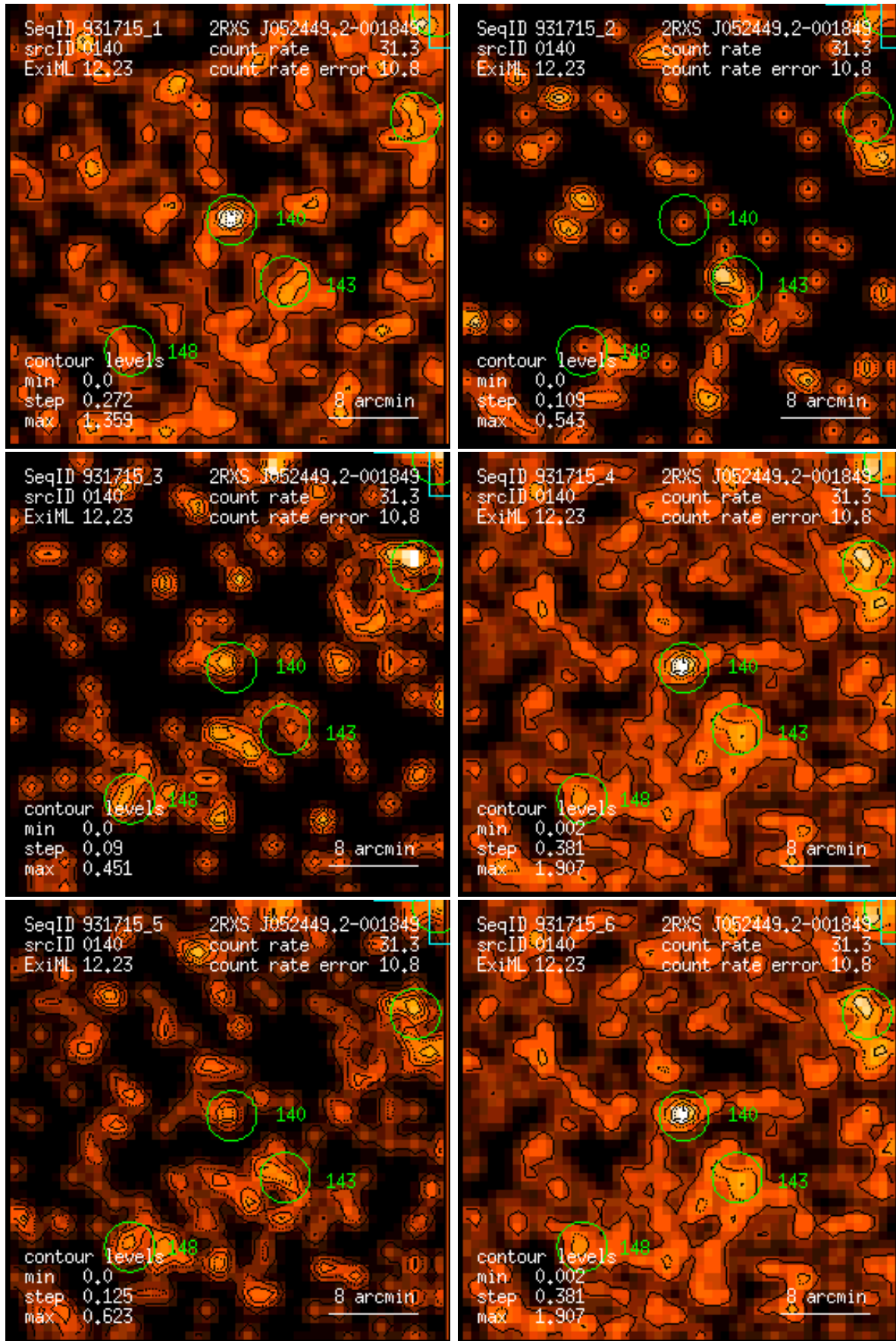
Figure 140: RASS 931715: detection 0140: band rate images, Gaussian filter: (1) PSPC channels 11 – 41, (2) 52 – 90, (3) 91 – 201, (4) 11 – 235, (5) 52 – 201, (6) 11 – 201. Broad band rates in counts/ks. Band rate contour levels in counts/ks/arcmin 2 .
