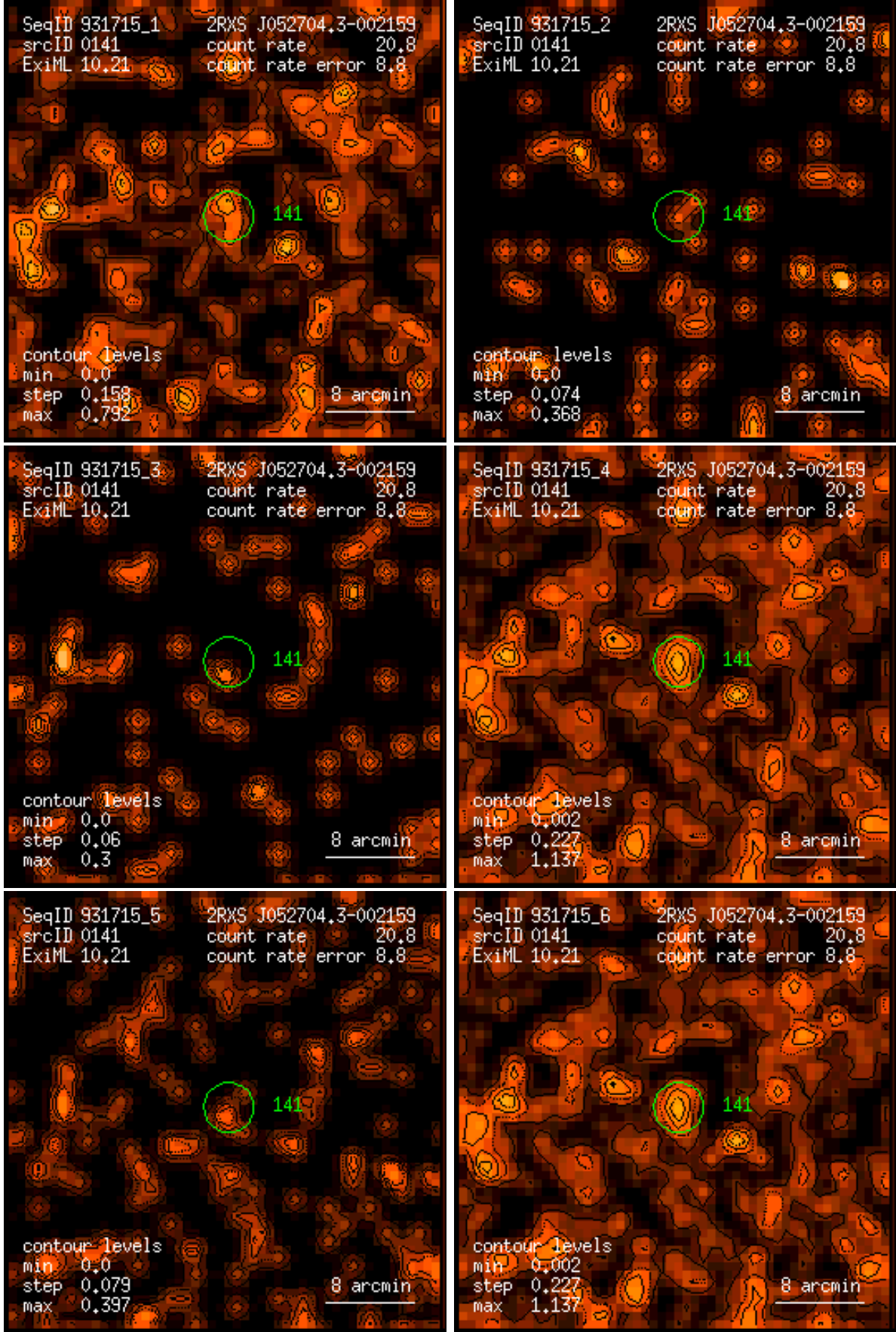
Figure 141: RASS 931715: detection 0141: band rate images, Gaussian filter: (1) PSPC channels 11 – 41, (2) 52 – 90, (3) 91 – 201, (4) 11 – 235, (5) 52 – 201, (6) 11 – 201. Broad band rates in counts/ks. Band rate contour levels in counts/ks/arcmin 2 .
