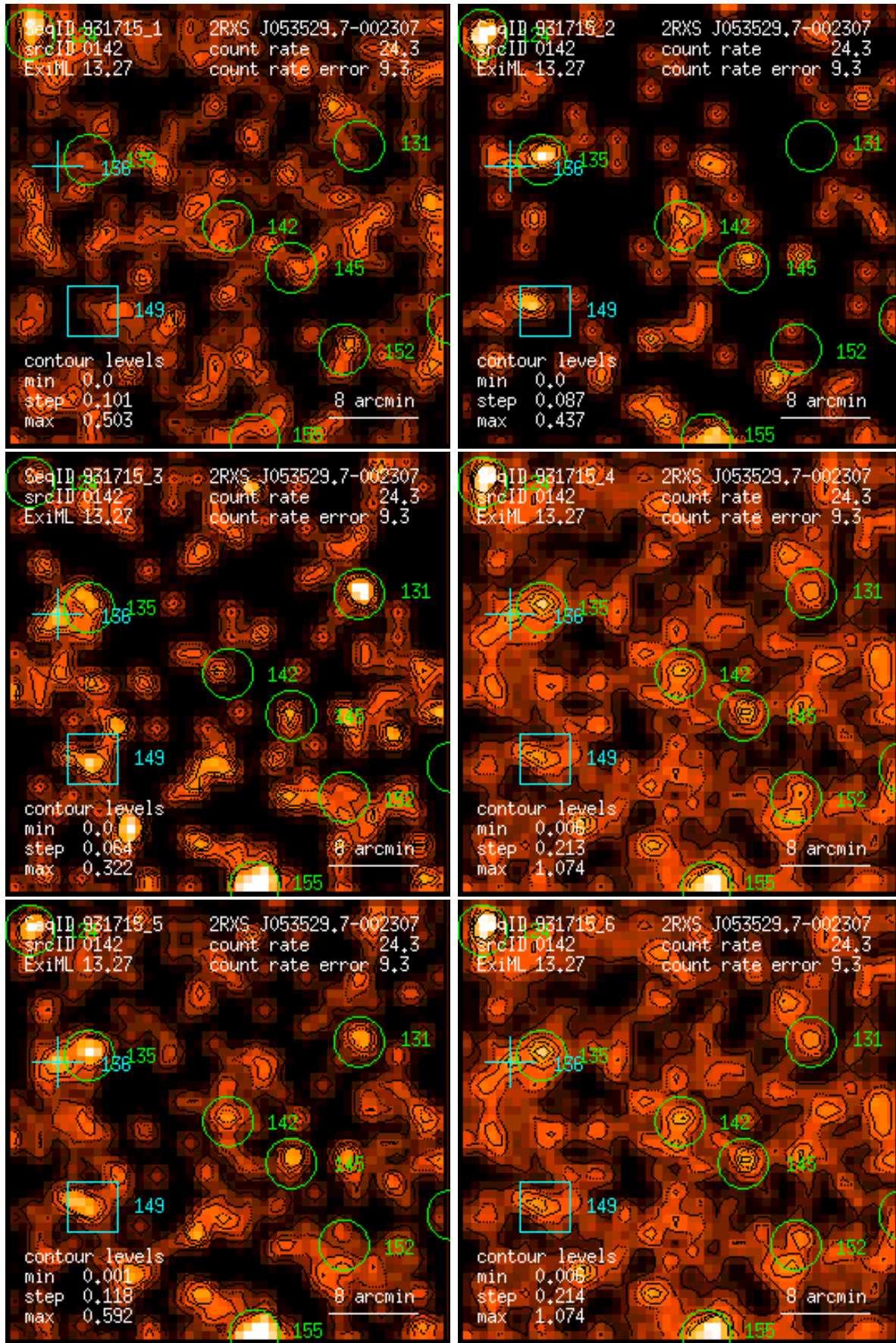
Figure 142: RASS 931715: detection 0142: band rate images, Gaussian filter: (1) PSPC channels 11 – 41, (2) 52 – 90, (3) 91 – 201, (4) 11 – 235, (5) 52 – 201, (6) 11 – 201. Broad band rates in counts/ks. Band rate contour levels in counts/ks/arcmin 2 .
