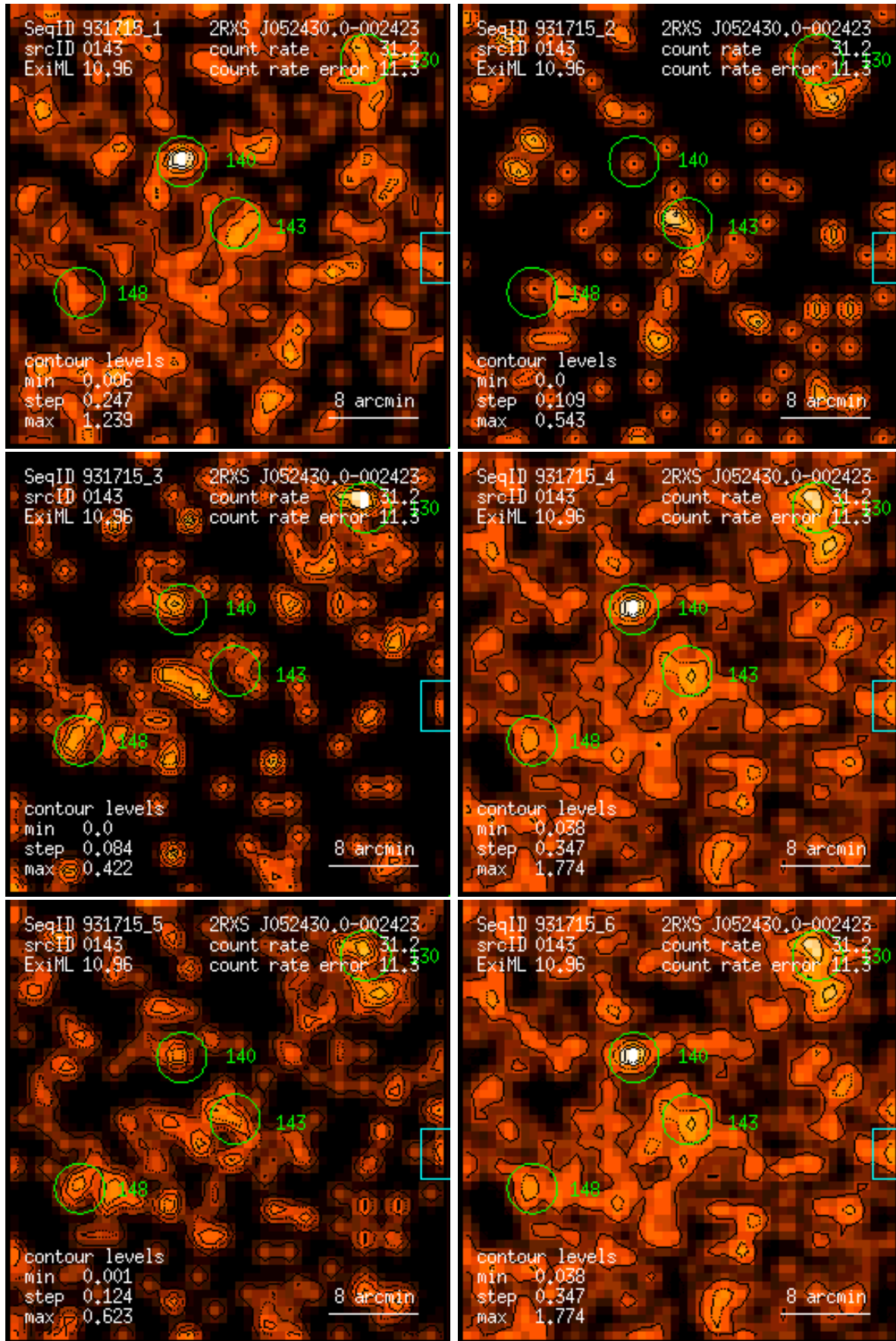
Figure 143: RASS 931715: detection 0143: band rate images, Gaussian filter: (1) PSPC channels 11 – 41, (2) 52 – 90, (3) 91 – 201, (4) 11 – 235, (5) 52 – 201, (6) 11 – 201. Broad band rates in counts/ks. Band rate contour levels in counts/ks/arcmin 2 .
