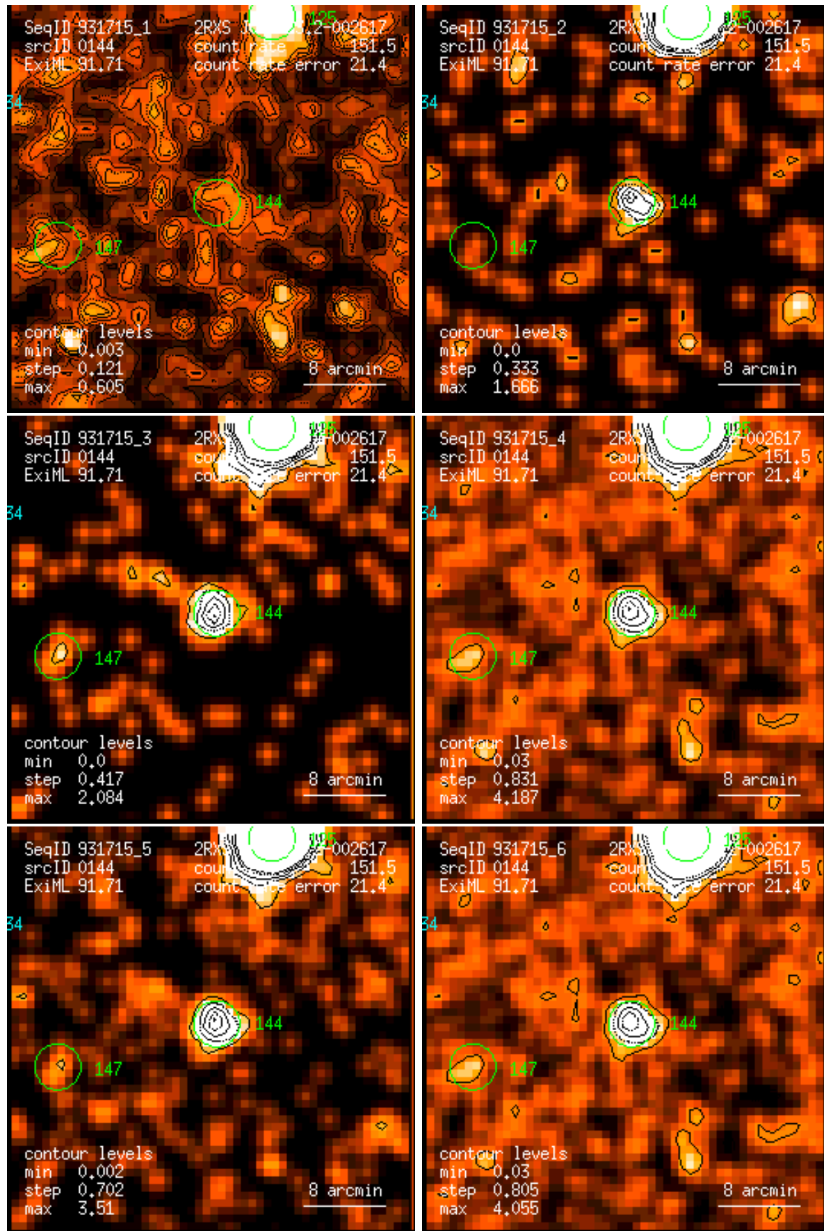
Figure 144: RASS 931715: detection 0144: band rate images, Gaussian filter: (1) PSPC channels 11 – 41, (2) 52 – 90, (3) 91 – 201, (4) 11 – 235, (5) 52 – 201, (6) 11 – 201. Broad band rates in counts/ks. Band rate contour levels in counts/ks/arcmin 2 .
